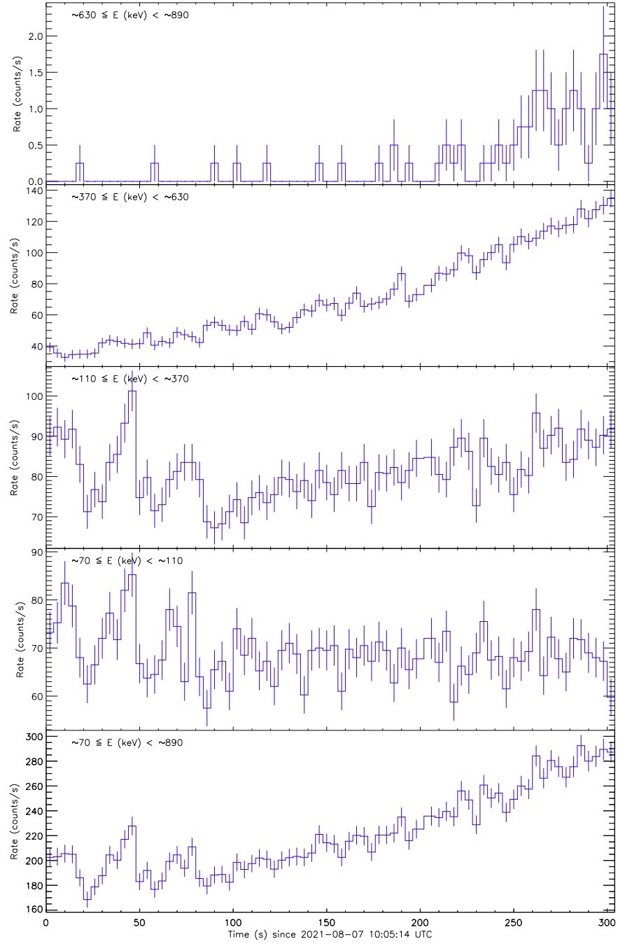
Figure 1: Raw count rate curve of GRB 210807A.
