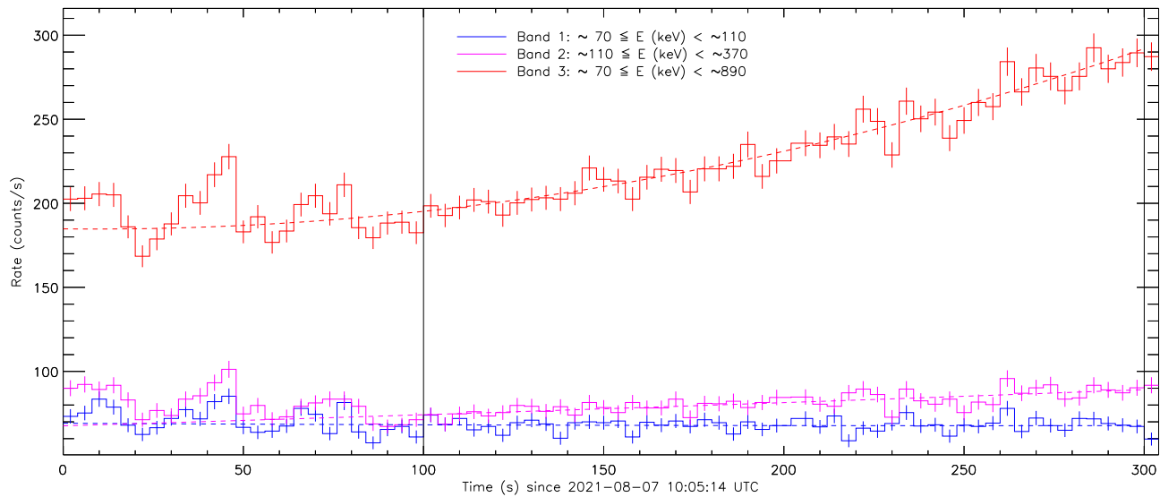
Figure 2: Background fit by a second order polynomial. Region used for the background fit is delimited by the two vertical solid lines.
