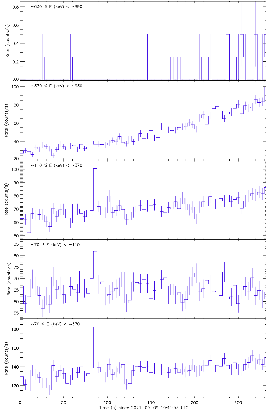
Figure 1: Raw count rate curve of GRB 210909A.
