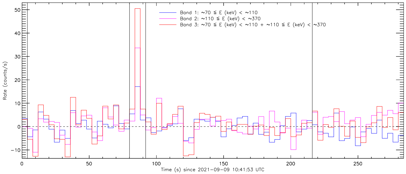
Figure 3: Background-subtracted count rate curve.
