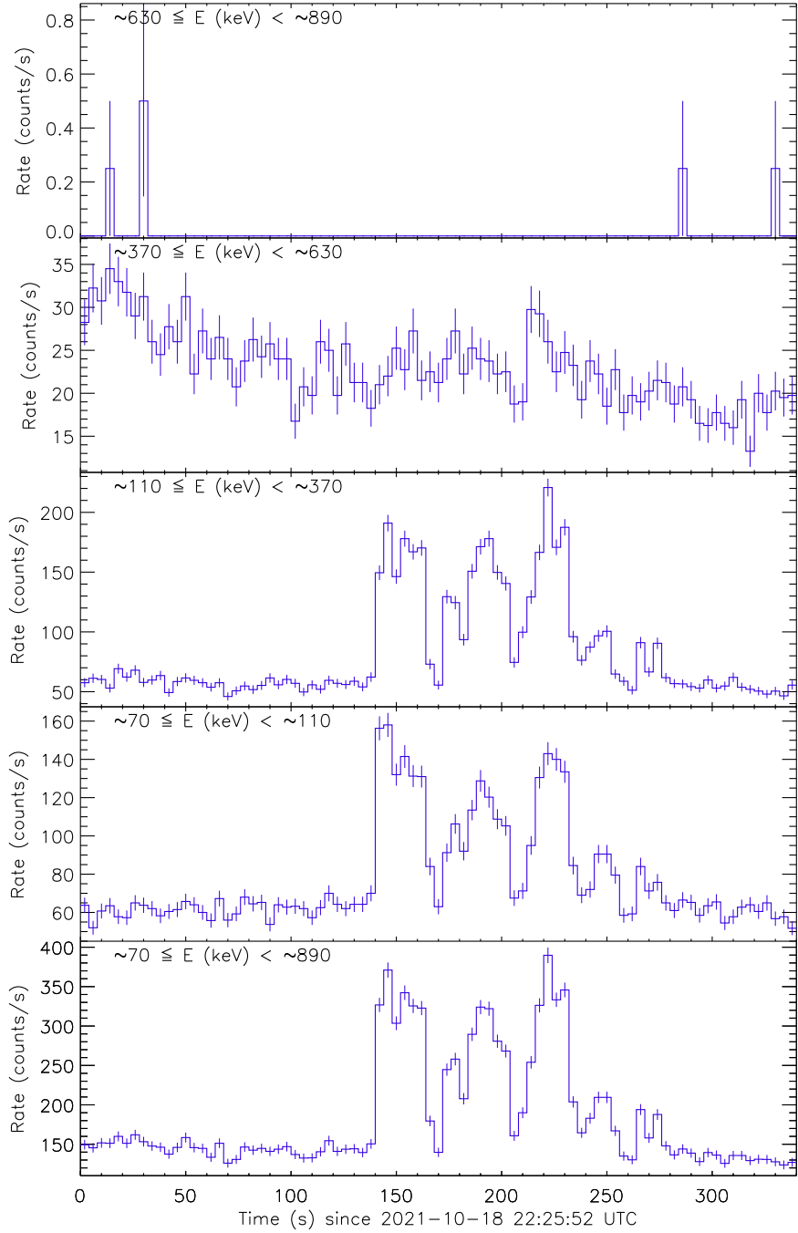
Figure 1: Raw count rate curve of GRB 211018A.
