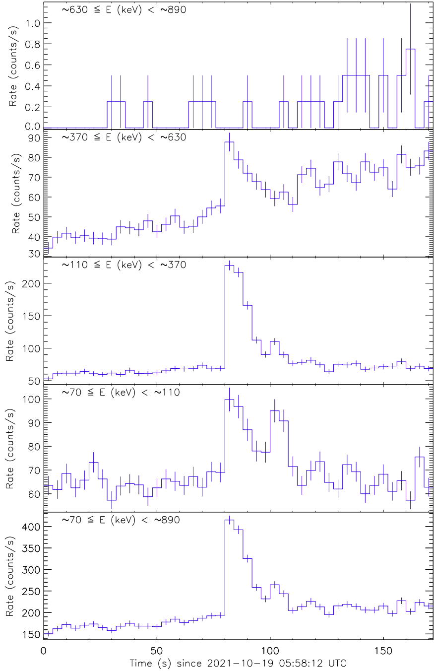
Figure 1: Raw count rate curve of GRB 211019A.
