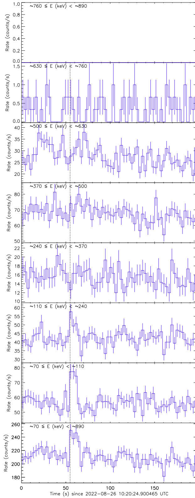
Figure 1: Raw count rate curve of GRB 220826B. The vertical dashed line marks the trigger time by Fermi/GBM.
