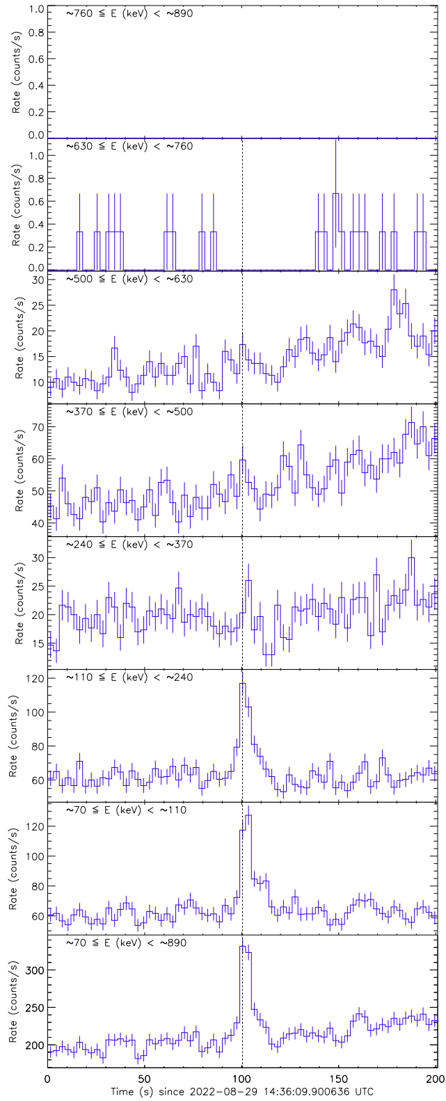
Figure 1: Raw count rate curve of GRB 220829A. The vertical dashed line marks the trigger time by Konus-Wind.
