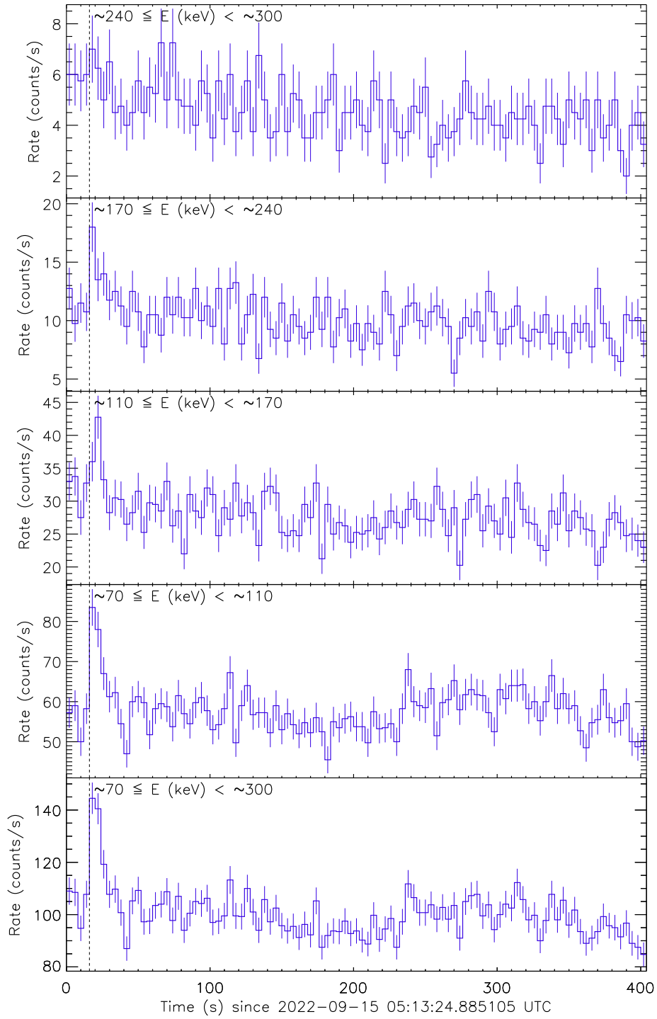
Figure 1: Raw count rate curve of GRB 220915A. The vertical dashed line marks the trigger time by Femi/GBM.
