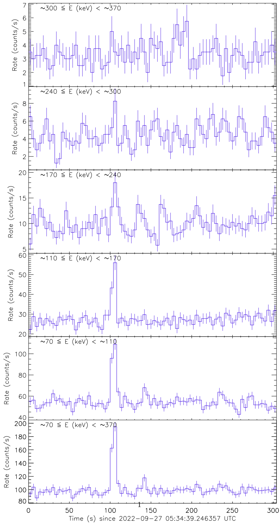
Figure 1: Raw count rate curve of GRB 220927A.
