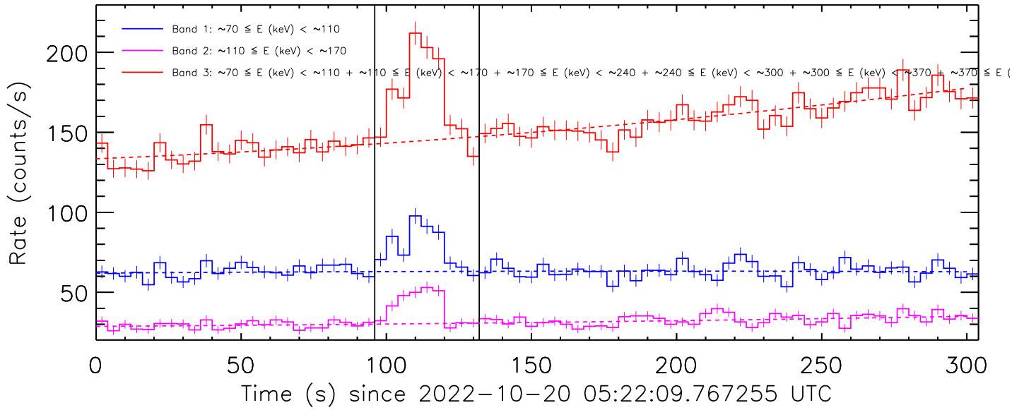
Figure 2: Background fit by a second order polynomial. Pre-burst and post-burst intervals which were used for the background fit are delimited by the vertical solid lines.
