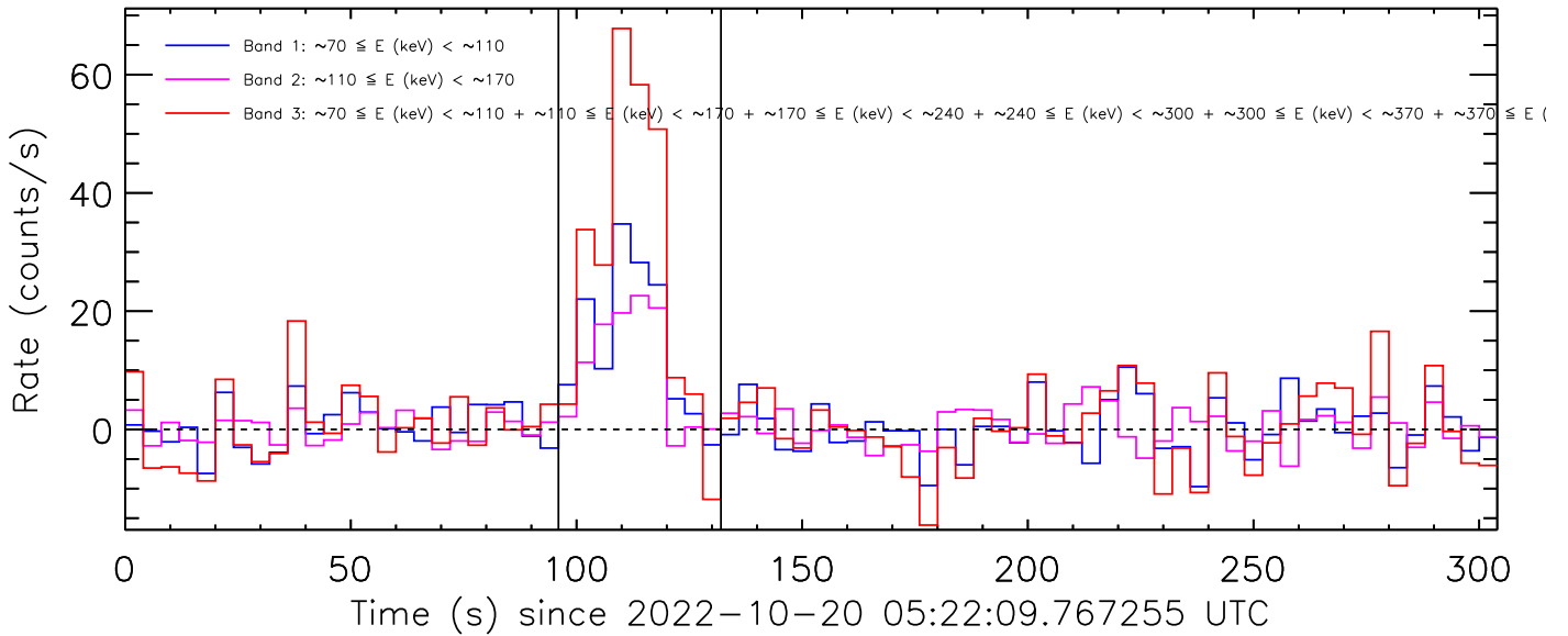
Figure 3: Background-subtracted count rate curves.
