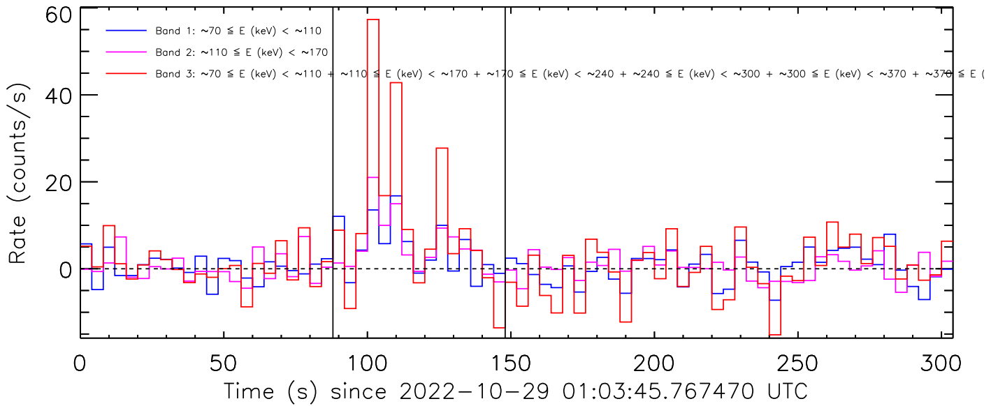
Figure 3: Background-subtracted count rate curves.
