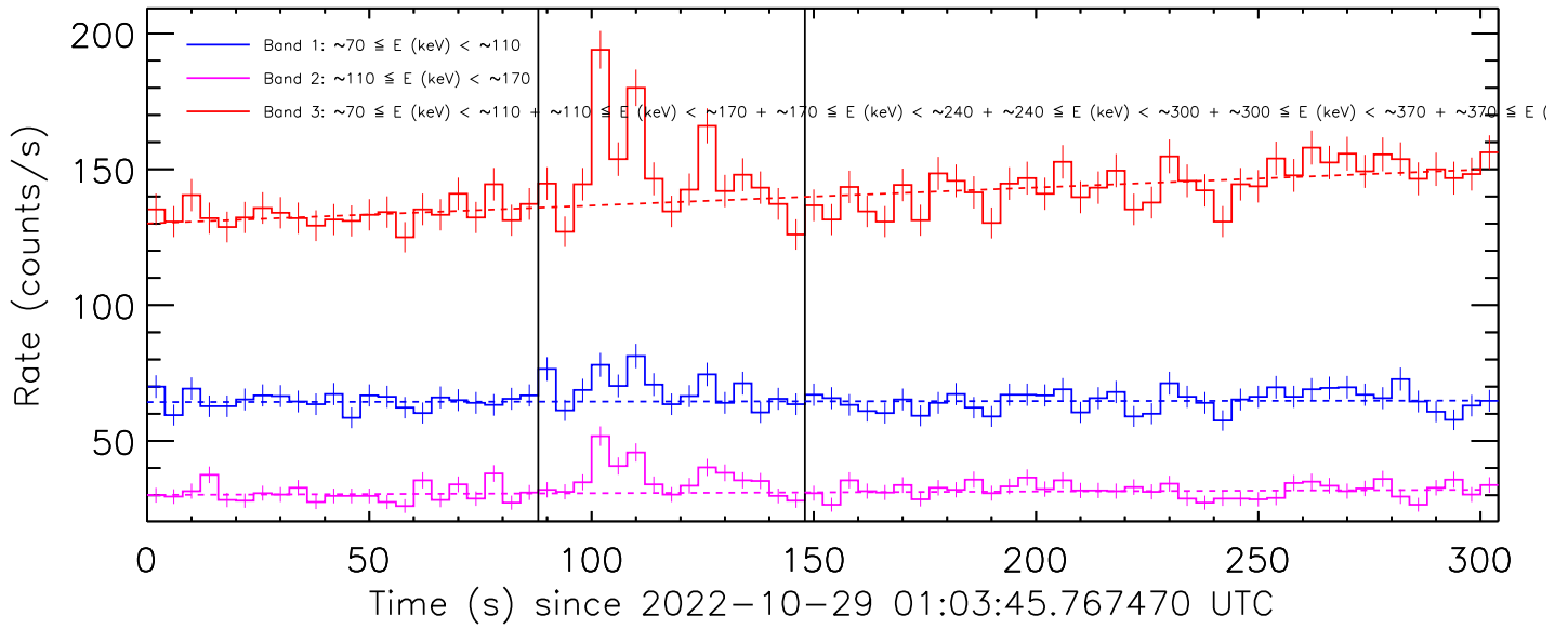
Figure 2: Background fit by a linear function. Pre-burst and post-burst intervals which were used for the background fit are delimited by the vertical solid lines.
