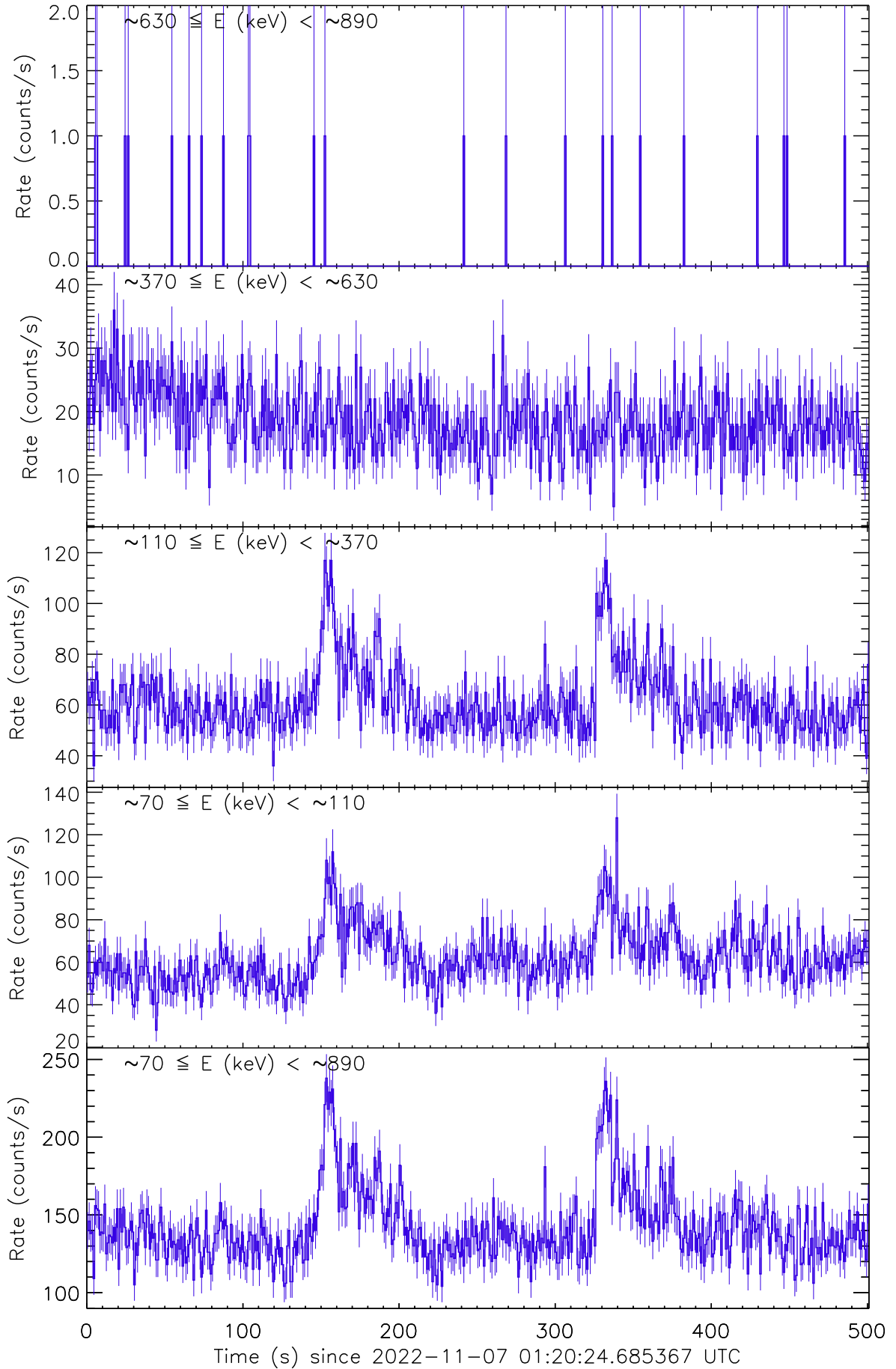
Figure 1: Raw count rate curve of GRB 221107A.
