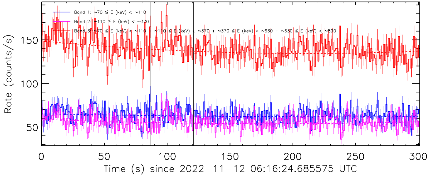
Figure 2: Background fit by a second order polynomial. Pre-burst and post-burst intervals were used for the background fit which are delimited by the vertical solid lines.
