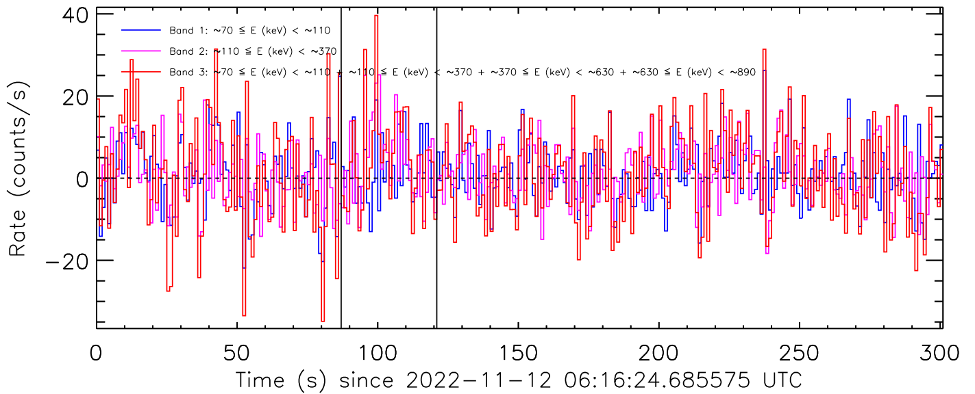
Figure 3: Background-subtracted count rate curve.
