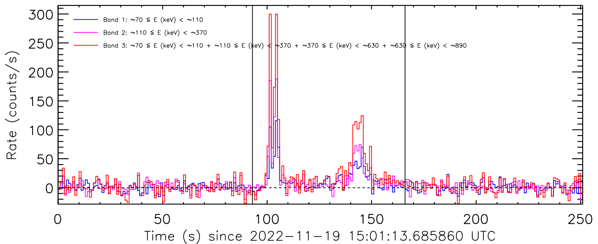
Figure 3: Background-subtracted count rate curve. Pre-burst and post-burst intervals were used for the background fit which are delimited by the vertical solid lines.
