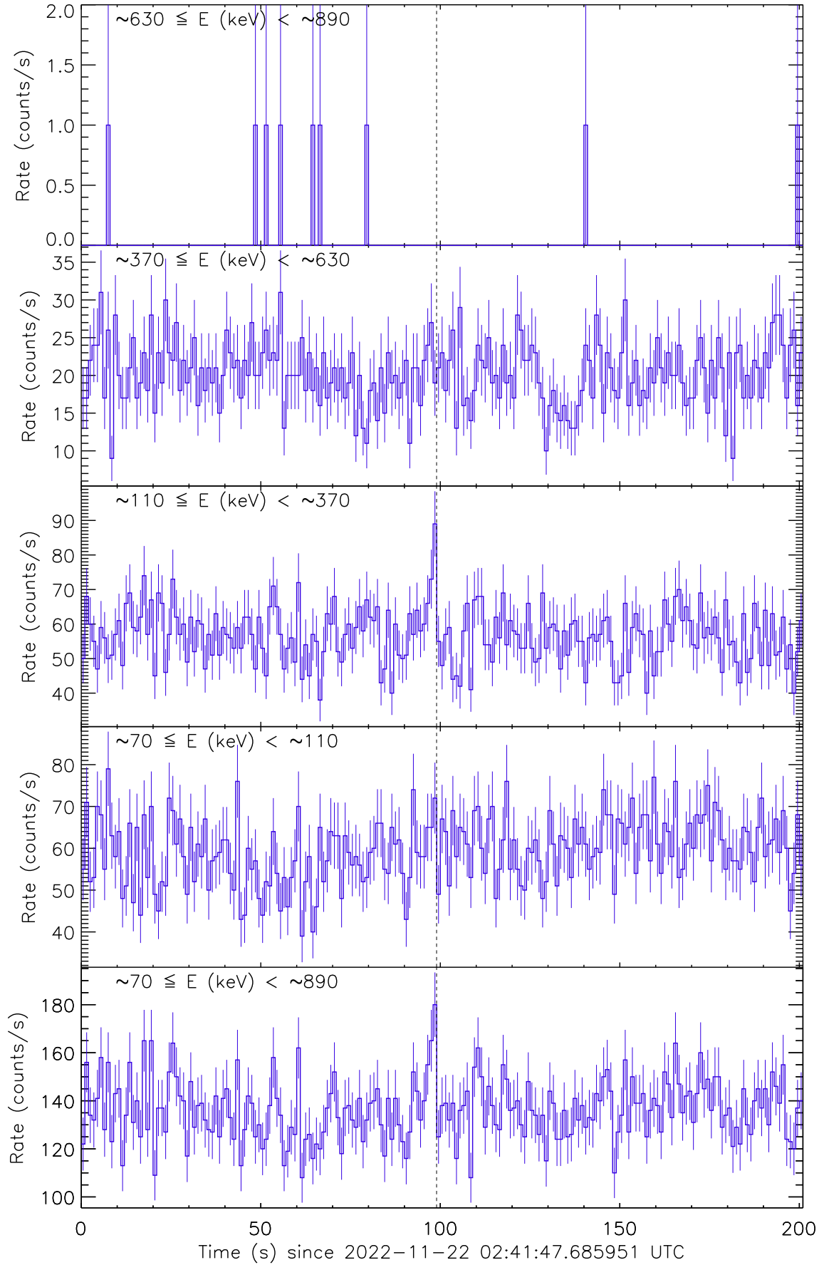
Figure 1: Raw count rate curve of GRB 221122A. The vertical dashed line marks the trigger time by GECAM-B.
