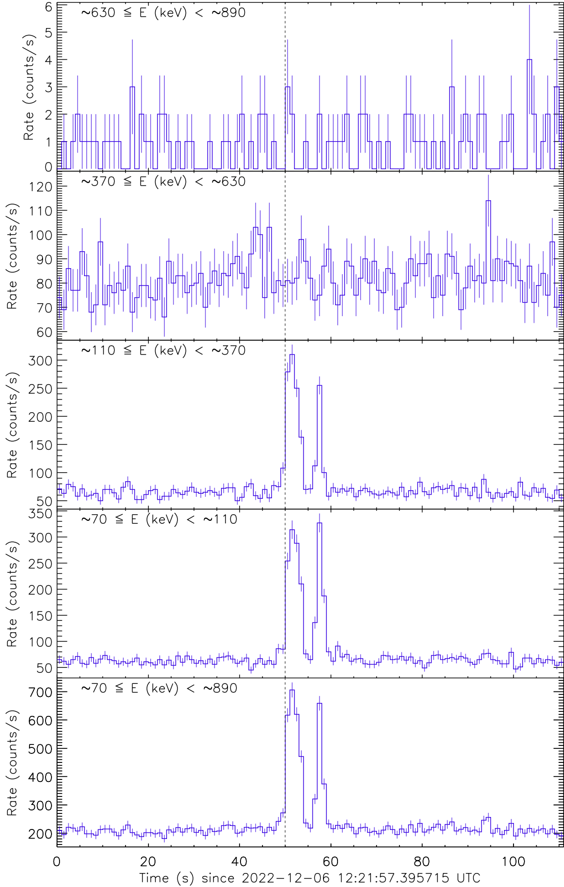
Figure 1: Raw count rate curve of GRB 221206B. The vertical dashed line marks the trigger time by Fermi/GBM.
