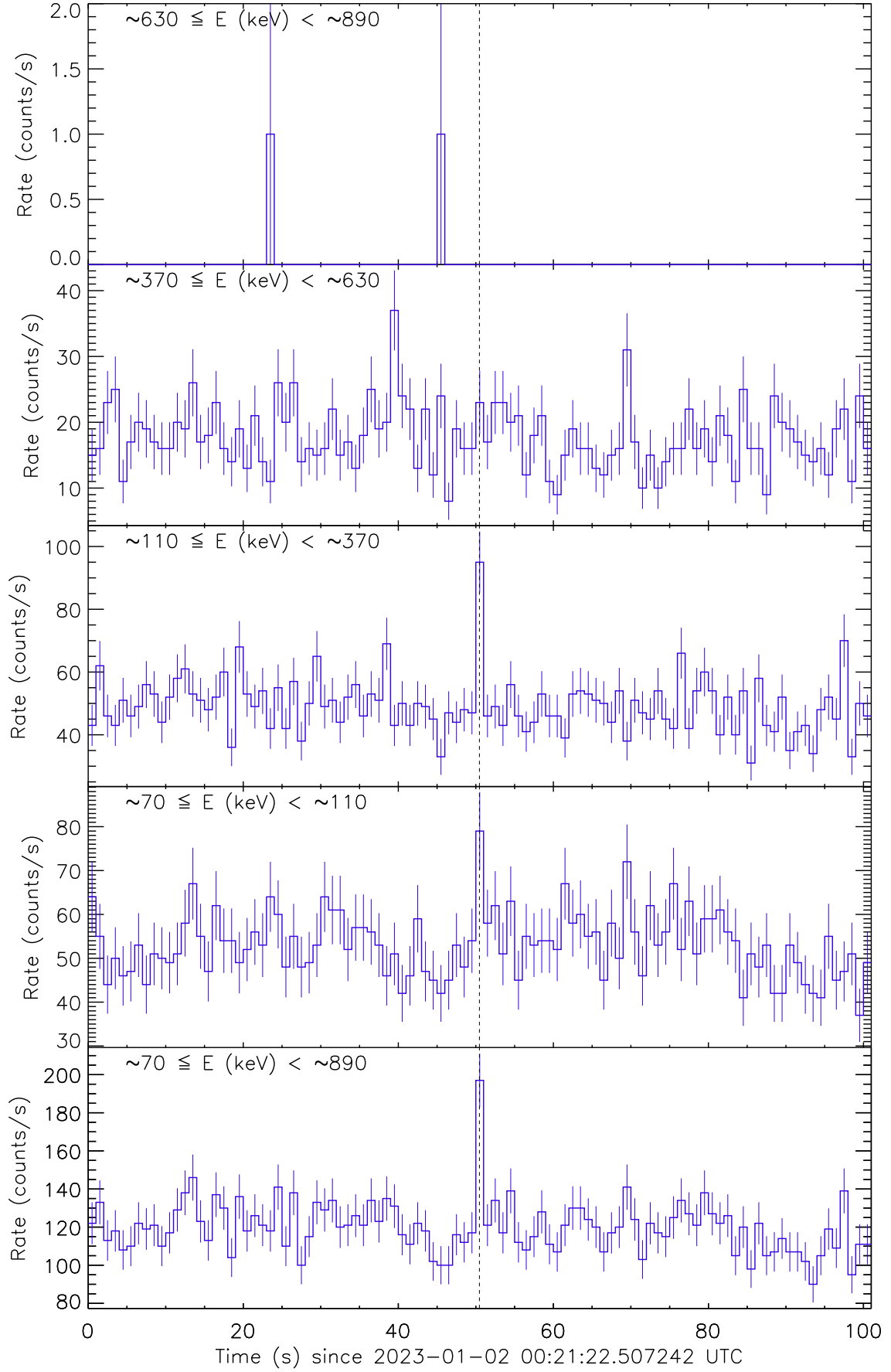
Figure 1: Raw count rate curve of GRB 230102A. The vertical dashed line marks the trigger time by Fermi/GBM.
