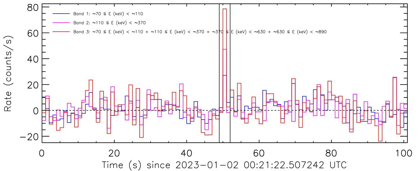
Figure 3: Background-subtracted count rate curve.
