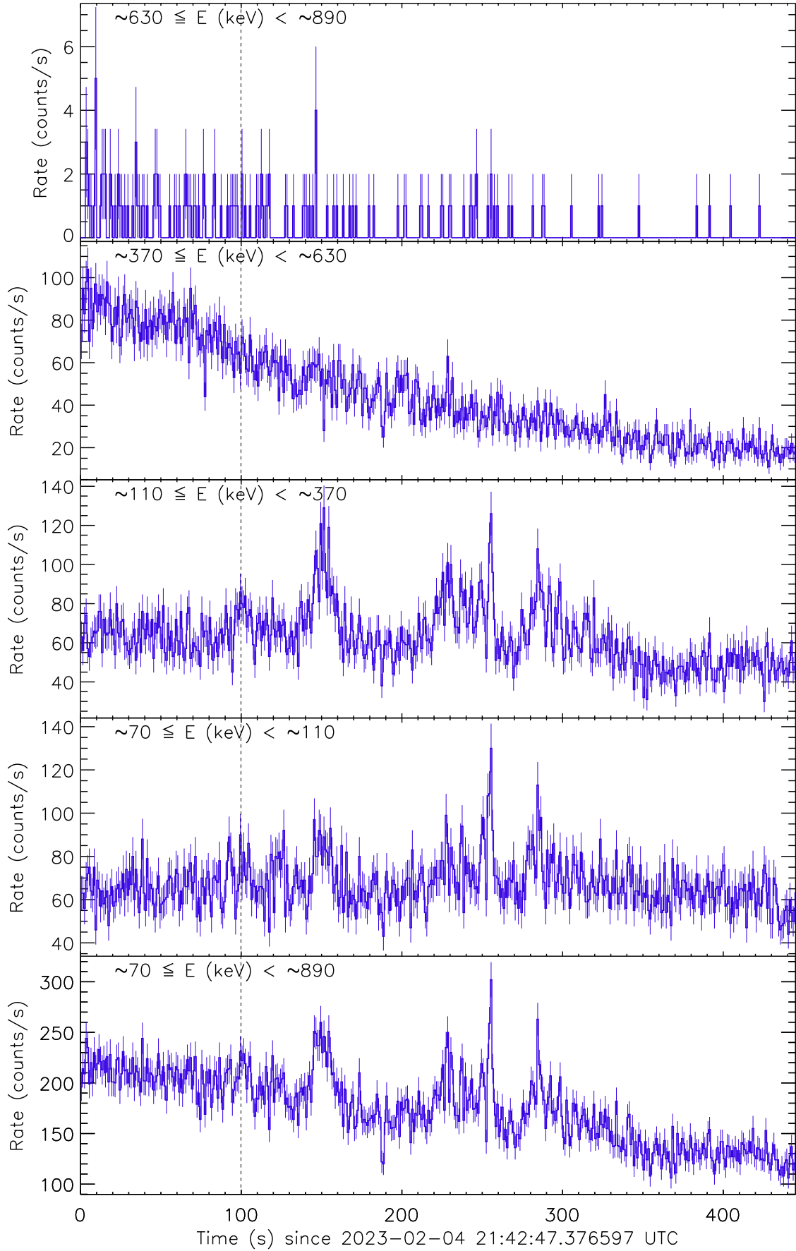
Figure 1: Raw count rate curve of GRB 230204B. The vertical dashed line marks the trigger time by Fermi/GBM.
