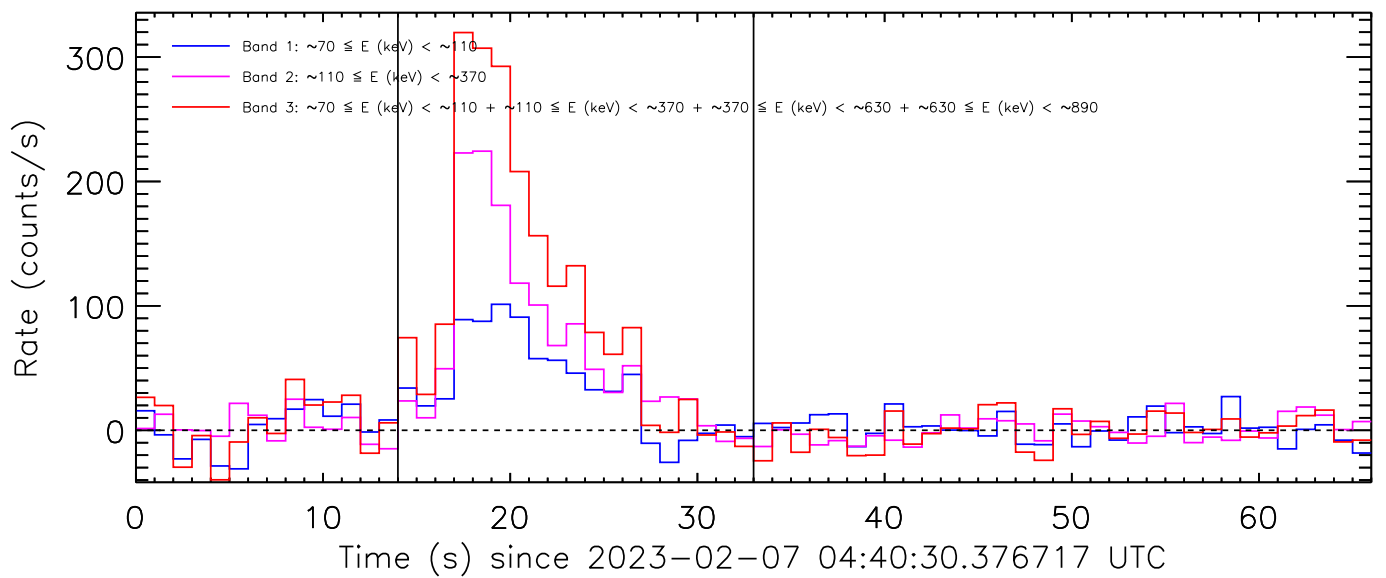
Figure 3: Background-subtracted count rate curve.
