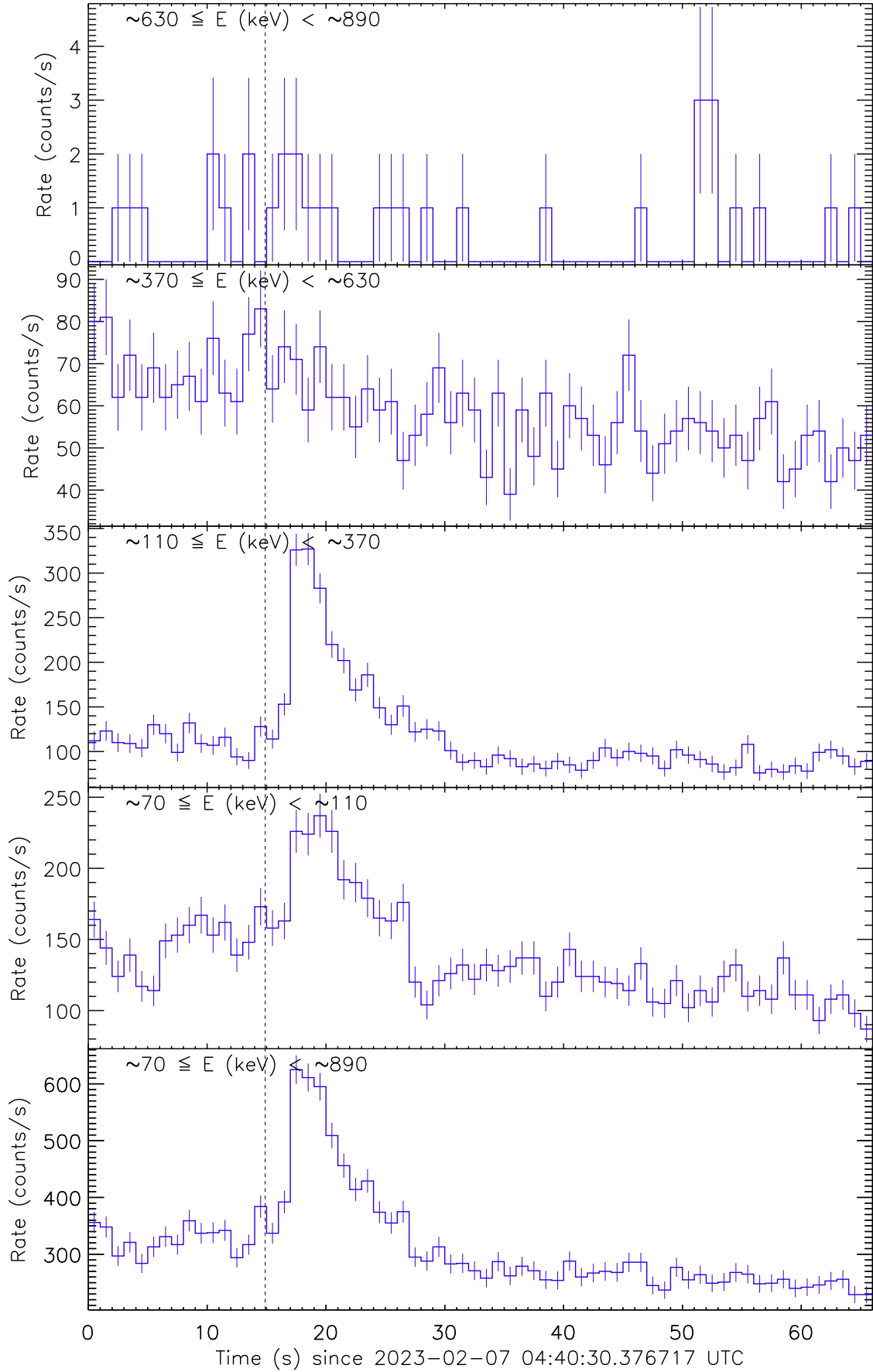
Figure 1: Raw count rate curve of GRB 230207B. The vertical dashed line marks the trigger time by INTEGRAL/SPI-ACS.
