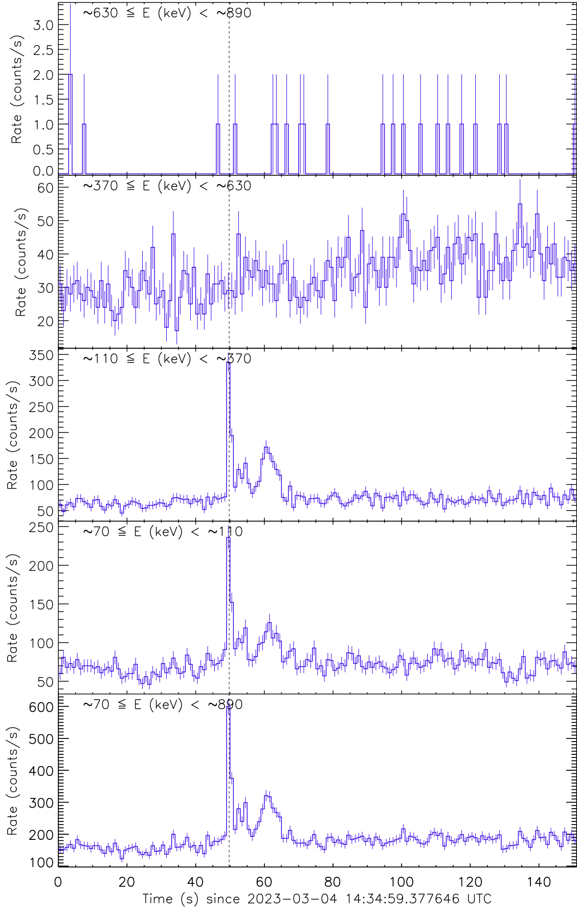
Figure 1: Raw count rate curve of GRB 230304B. The vertical dashed line marks the trigger time by Fermi/GBM.
