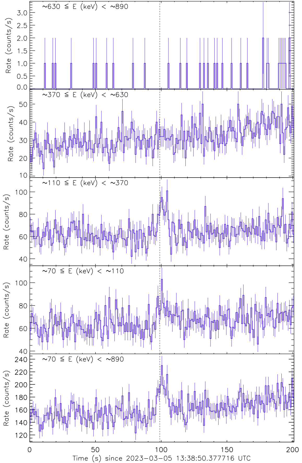
Figure 1: Raw count rate curve of GRB 230305A. The vertical dashed line marks the trigger time by Fermi/GBM.
