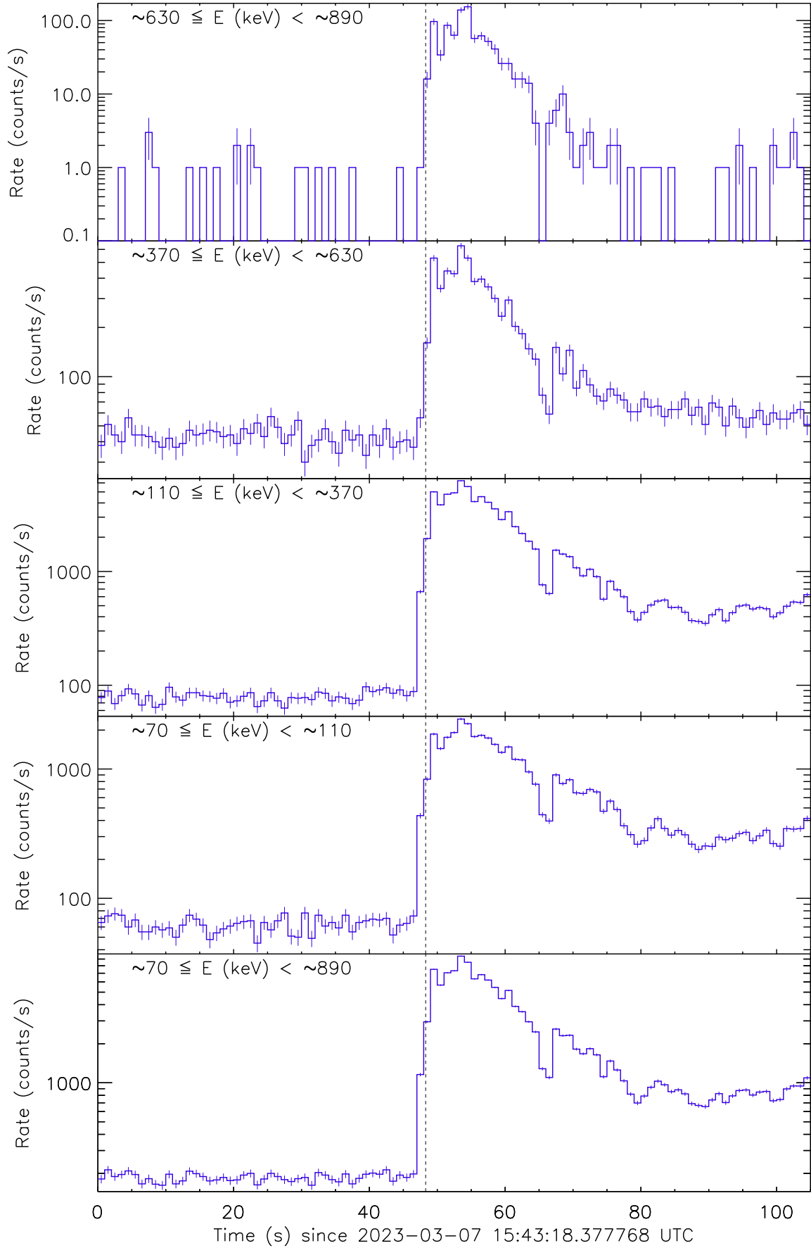
Figure 1: Raw count rate curve of GRB 230307A. The vertical dashed line marks the trigger time by Fermi/GBM.
