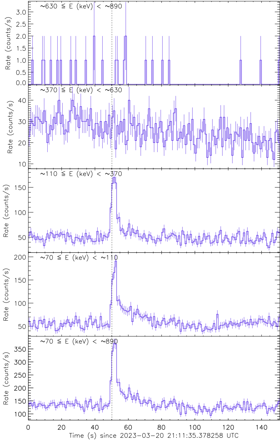
Figure 1: Raw count rate curve of GRB 230320B. The vertical dashed line marks the trigger time by Fermi/GBM.
