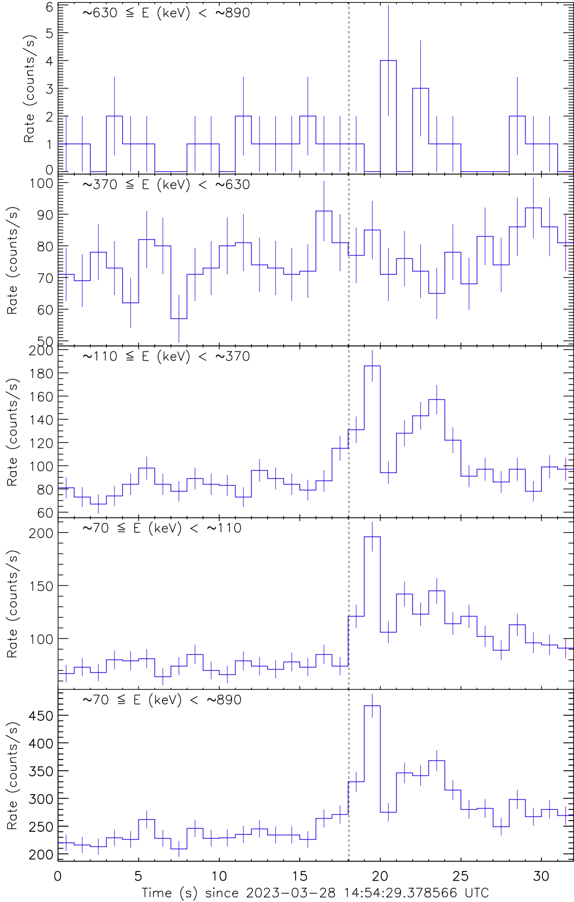
Figure 1: Raw count rate curve of GRB 230328B. The vertical dashed line marks the trigger time by Fermi/GBM.
