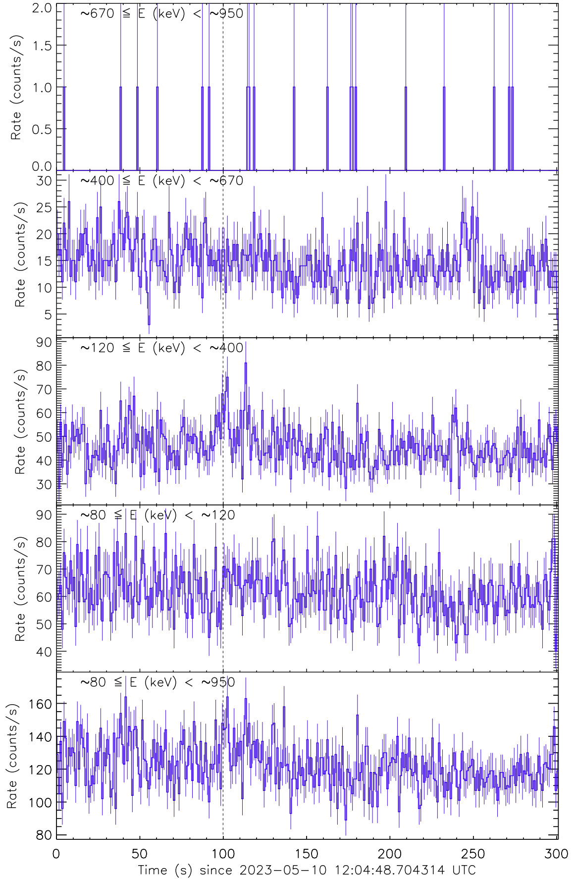
Figure 1: Raw count rate curve of GRB 230510A. The vertical dashed line marks the trigger time by Swift/BAT.
