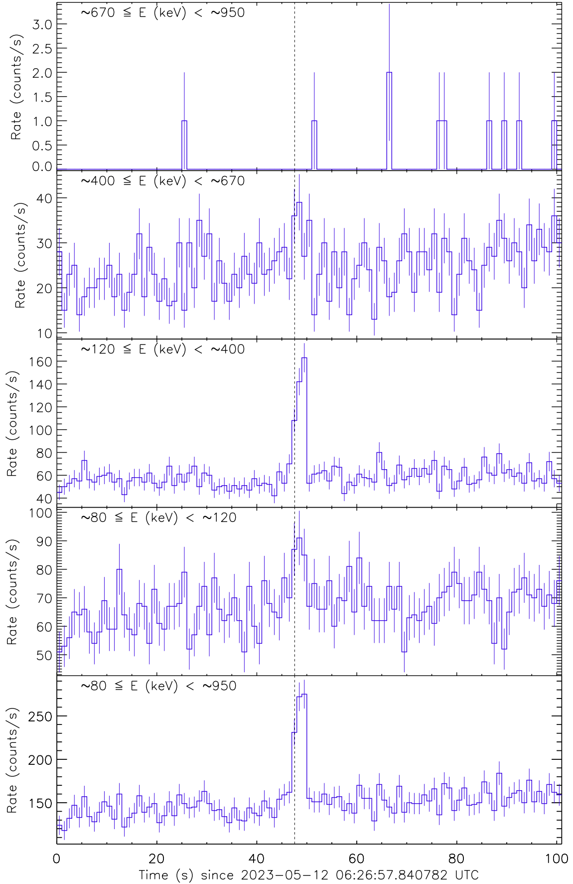
Figure 1: Raw count rate curve of GRB 230512A. The vertical dashed line marks the trigger time by Fermi/GBM.
