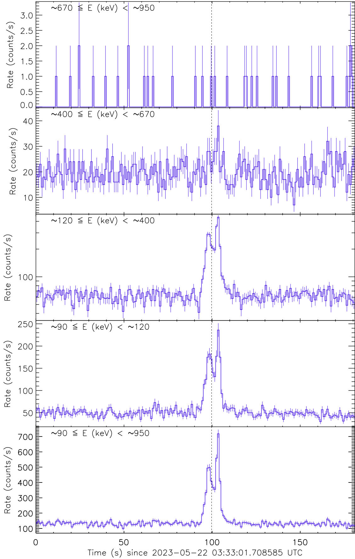
Figure 1: Raw count rate curve of GRB 230522A. The vertical dashed line marks the trigger time by Konus/Wind.
