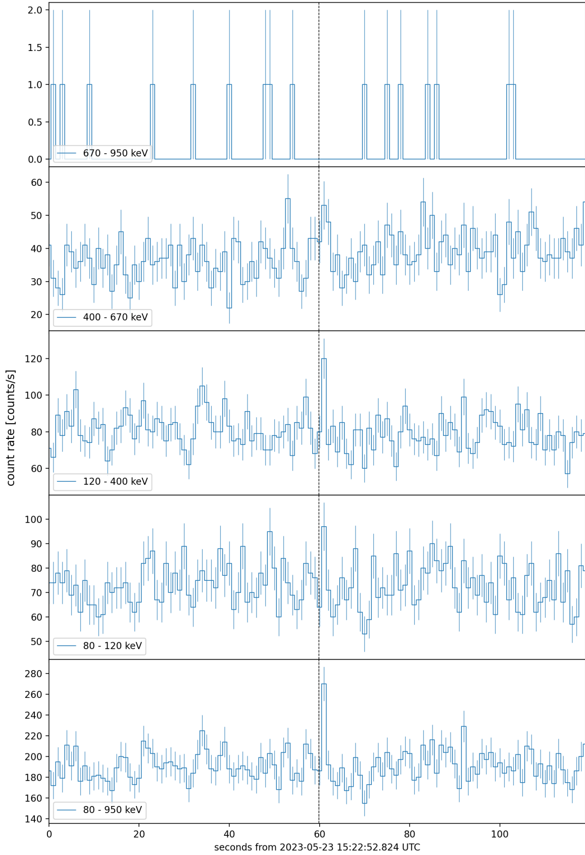
Figure 1: Raw count rate curve of GRB 230523B. The vertical dashed line marks the trigger time by INTEGRAL/SPI-ACS.
