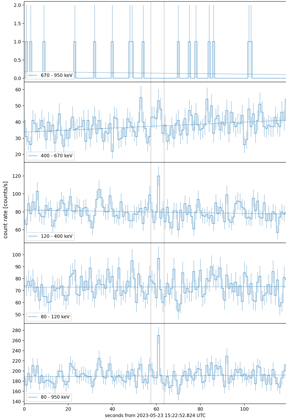
Figure 2: Background fit by a linear function. Pre-burst and post-burst intervals were used for the background fit which are delimited by the vertical solid lines.
