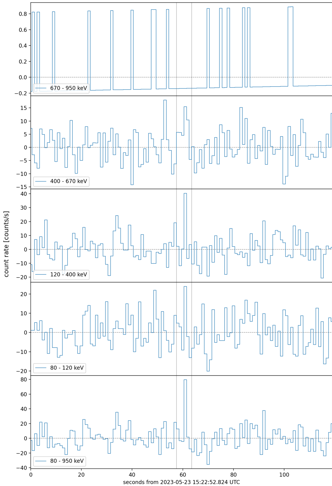
Figure 3: Background-subtracted count rate curve.
