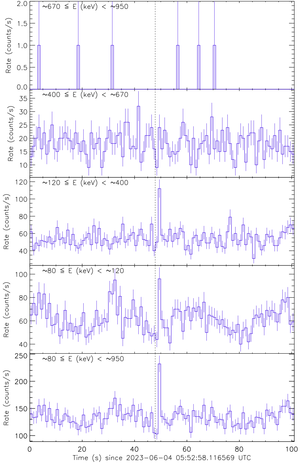
Figure 1: Raw count rate curve of GRB 230604A. The vertical dashed line marks the trigger time by AstroSat.
