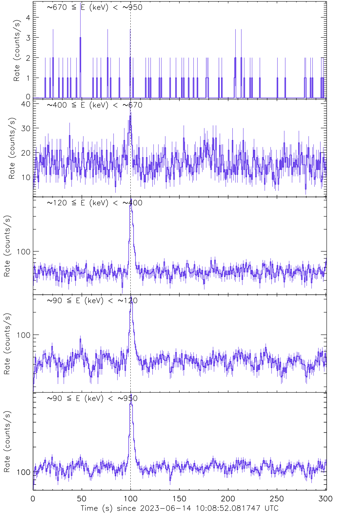
Figure 1: Raw count rate curve of GRB 230614C. The vertical dashed line marks the trigger time by Fermi/GBM.
