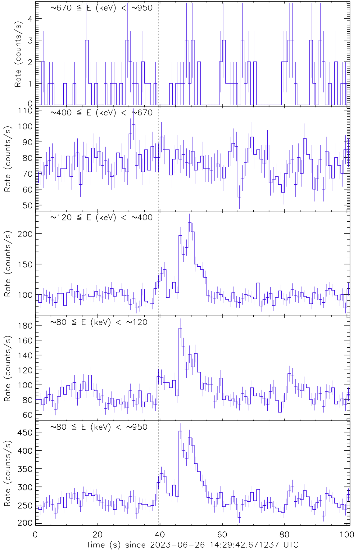
Figure 1: Raw count rate curve of GRB 230626A. The vertical dashed line marks the trigger time by Fermi/GBM.
