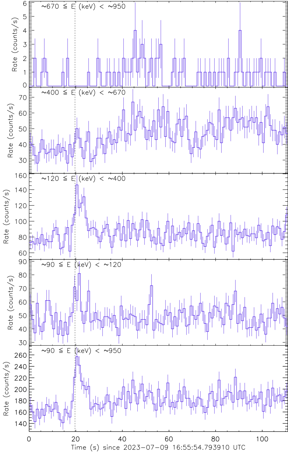
Figure 1: Raw count rate curve of GRB 230709B. The vertical dashed line marks the trigger time by Fermi/GBM.
