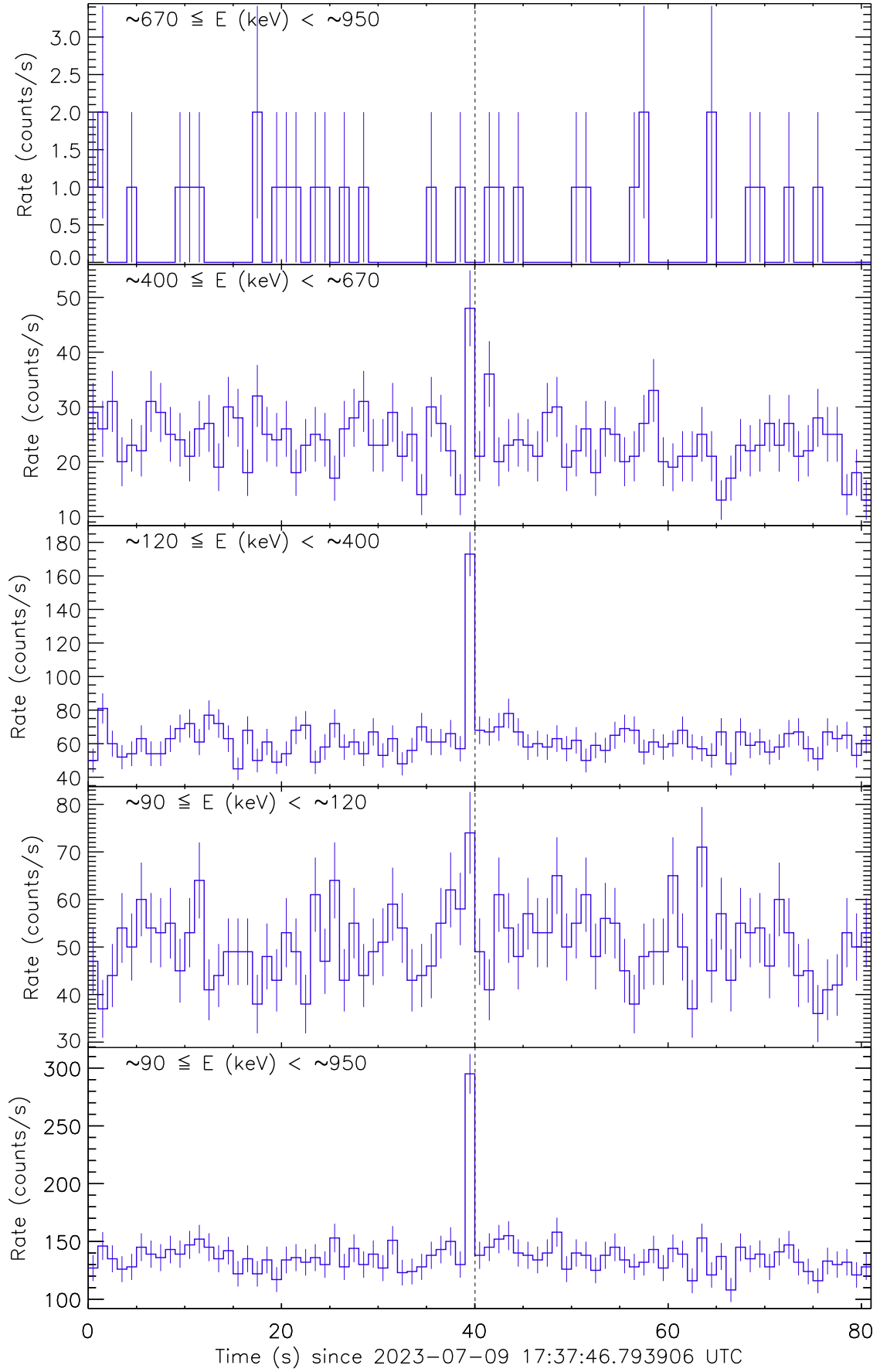
Figure 1: Raw count rate curve of GRB 230709C. The vertical dashed line marks the trigger time by Fermi/GBM.
