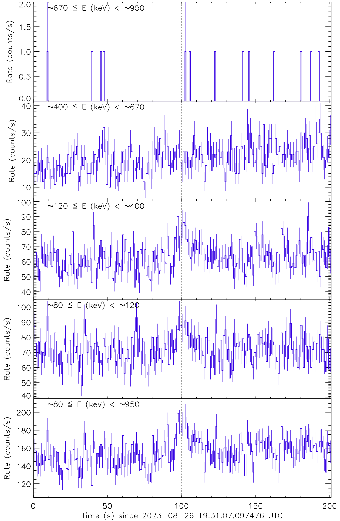
Figure 1: Raw count rate curve of GRB 230826A. The vertical dashed line marks the trigger time by Swift/BAT.
