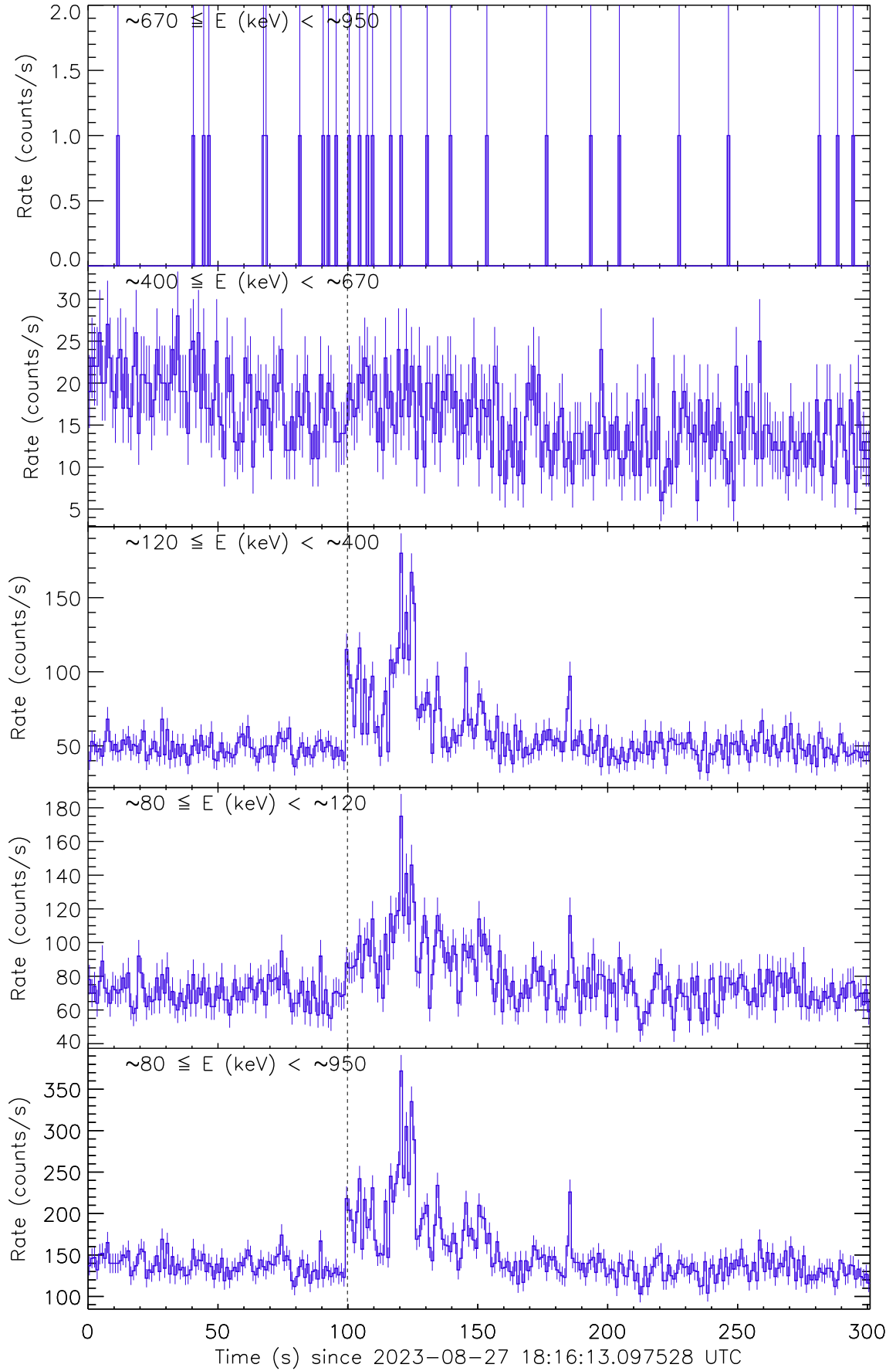
Figure 1: Raw count rate curve of GRB 230827A. The vertical dashed line marks the trigger time by Fermi/GBM.
