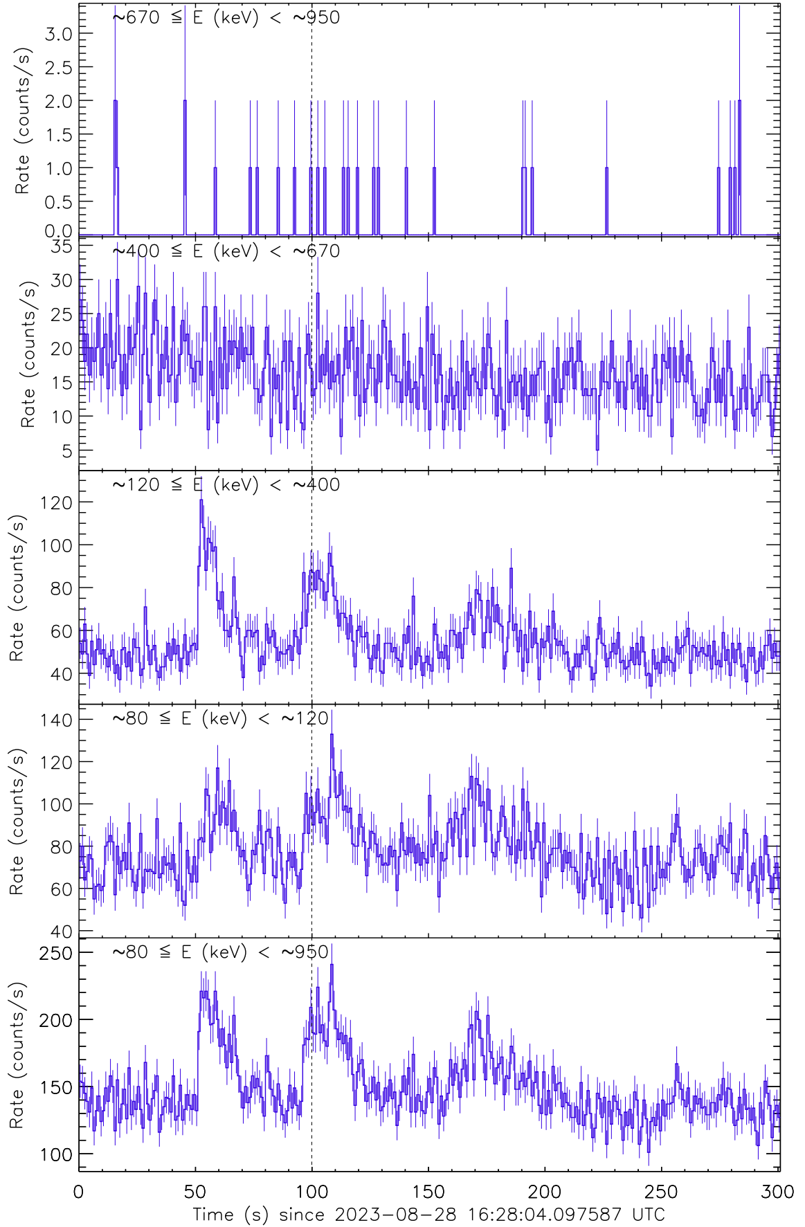
Figure 1: Raw count rate curve of GRB 230828A. The vertical dashed line marks the trigger time by AstroSat.
