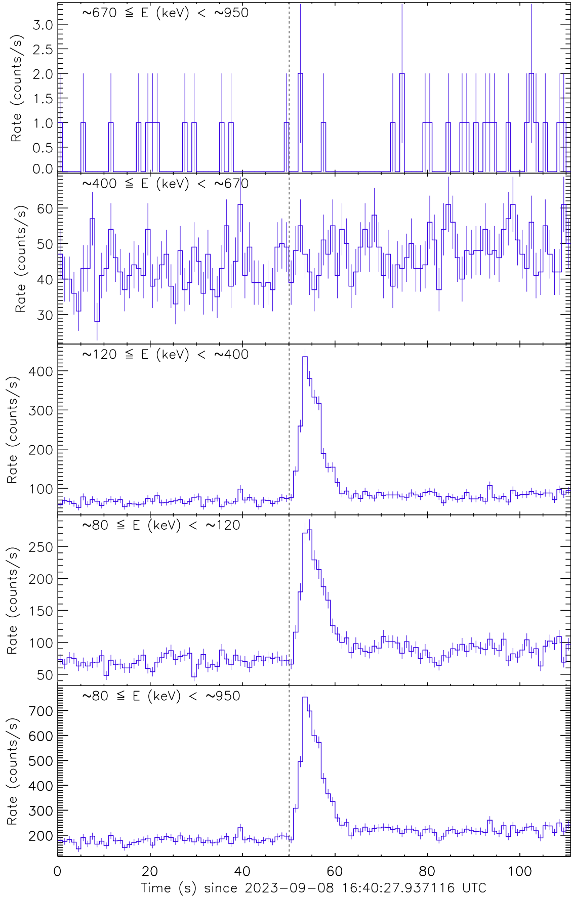
Figure 1: Raw count rate curve of GRB 230908A. The vertical dashed line marks the trigger time by AstroSat.
