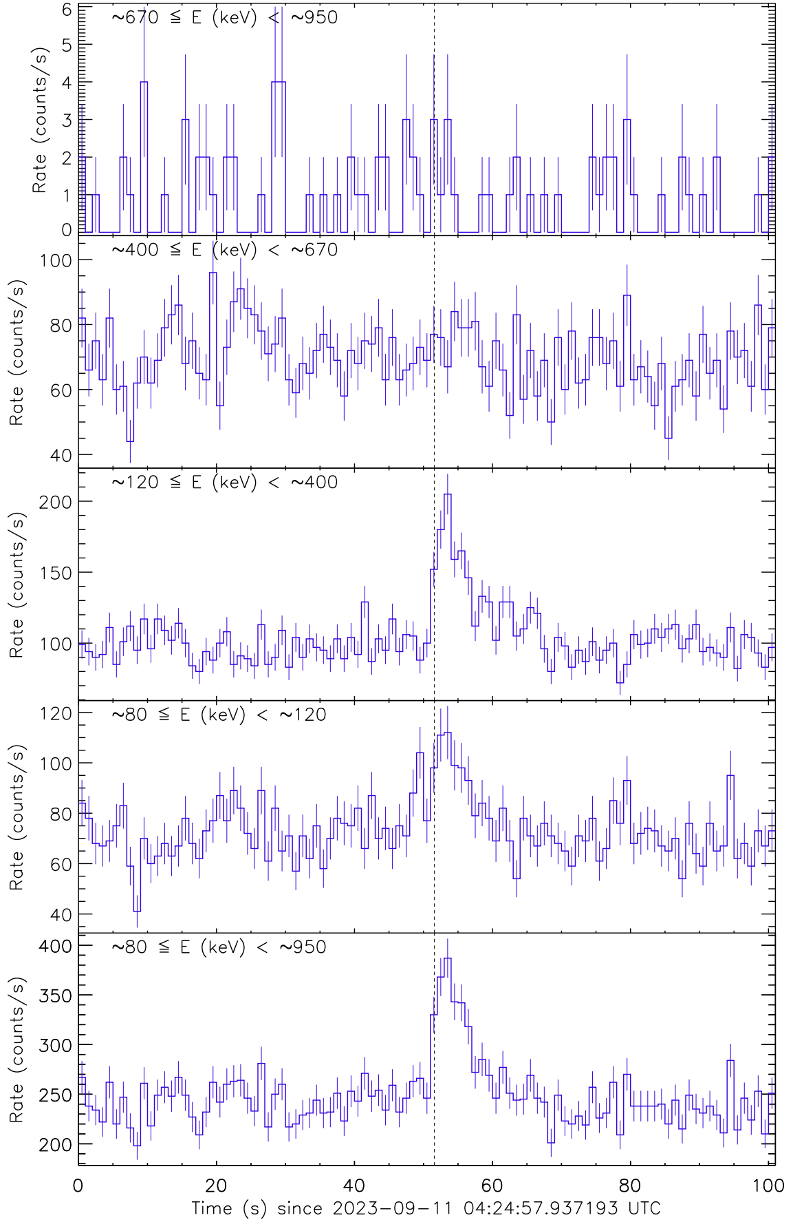
Figure 1: Raw count rate curve of GRB 230911B. The vertical dashed line marks the trigger time by Fermi/GBM.
