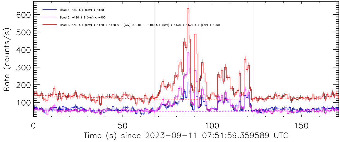
Figure 2: Background fit by a second-order polynomial. Pre-burst and post-burst intervals were used for the background fit which are delimited by the vertical solid lines.
