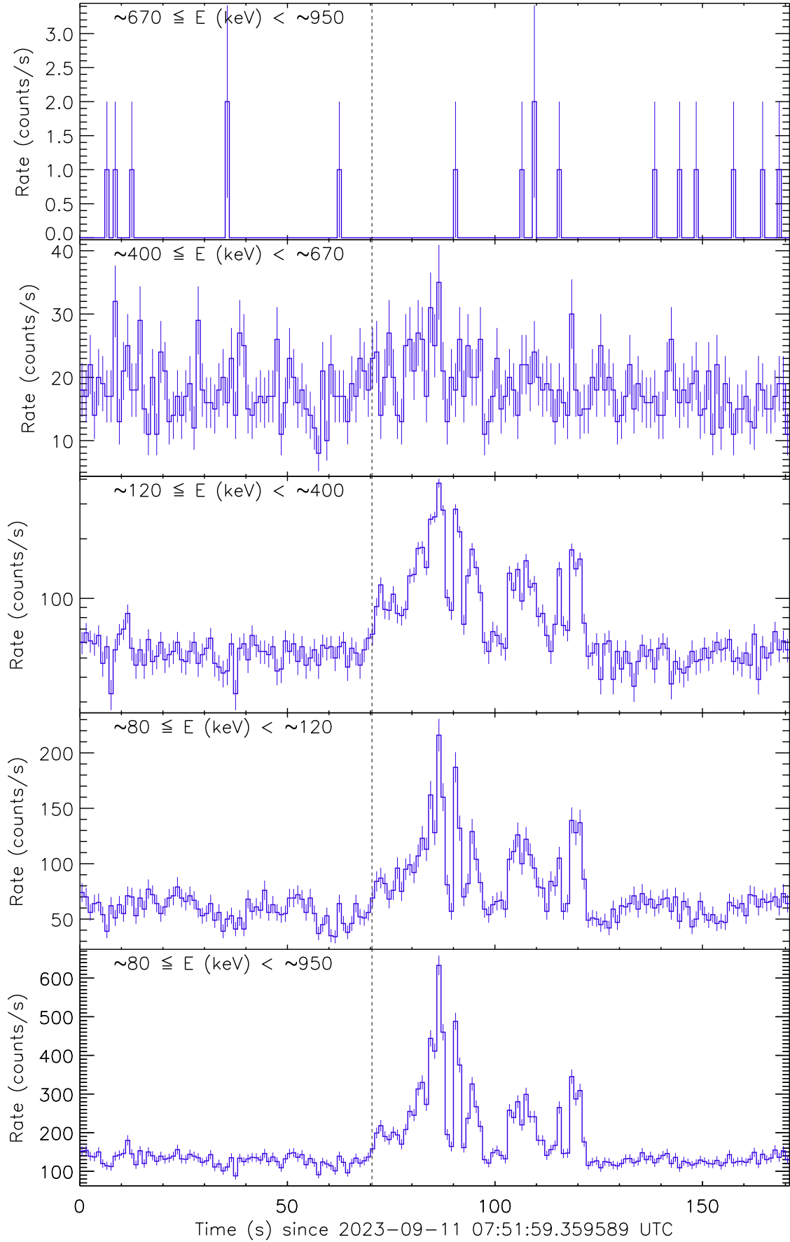
Figure 1: Raw count rate curve of GRB 230911D. The vertical dashed line marks the trigger time by Fermi/GBM.
