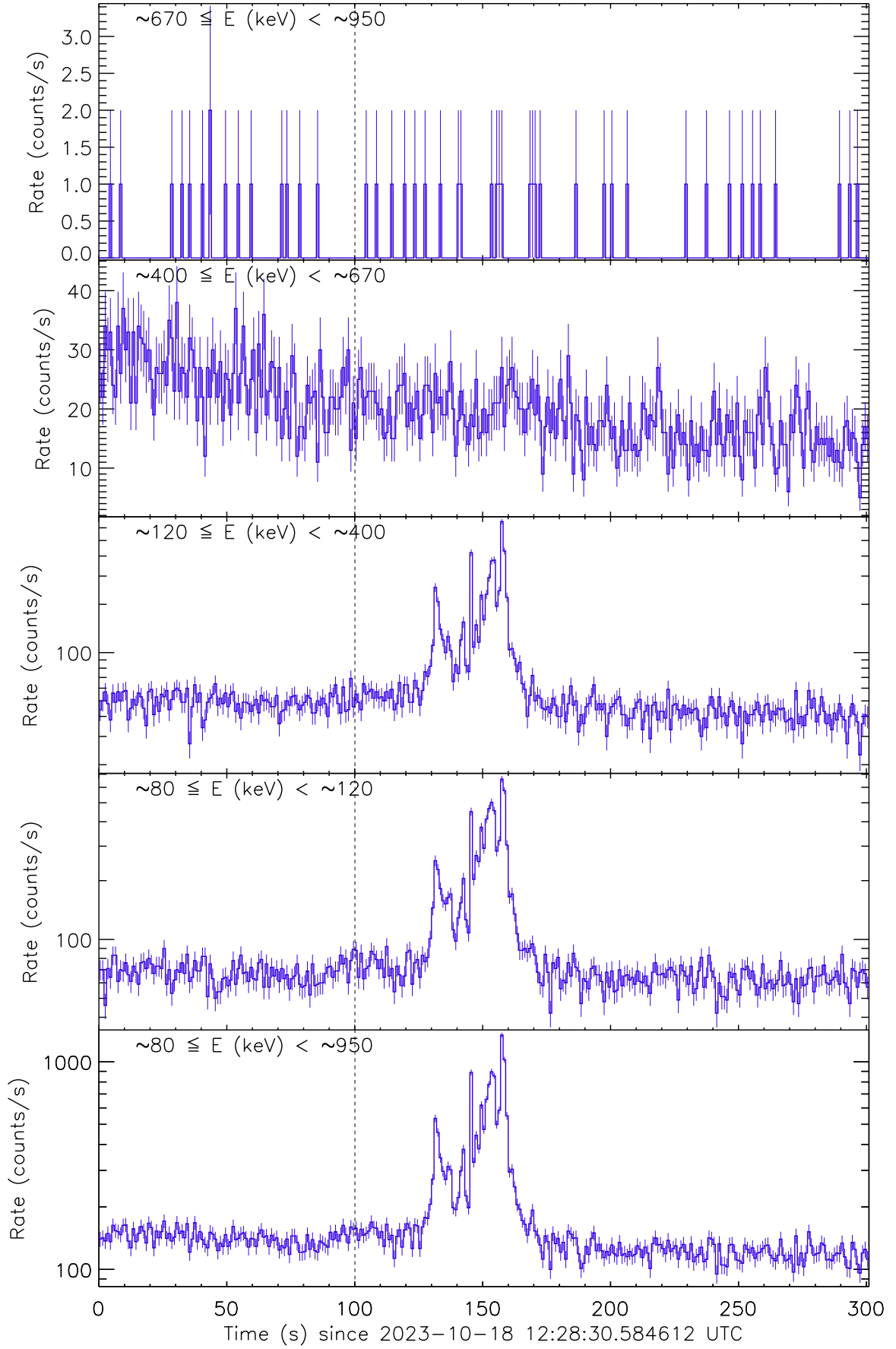
Figure 1: Raw count rate curve of GRB 231018A. The vertical dashed line marks the trigger time by Fermi/GBM.
