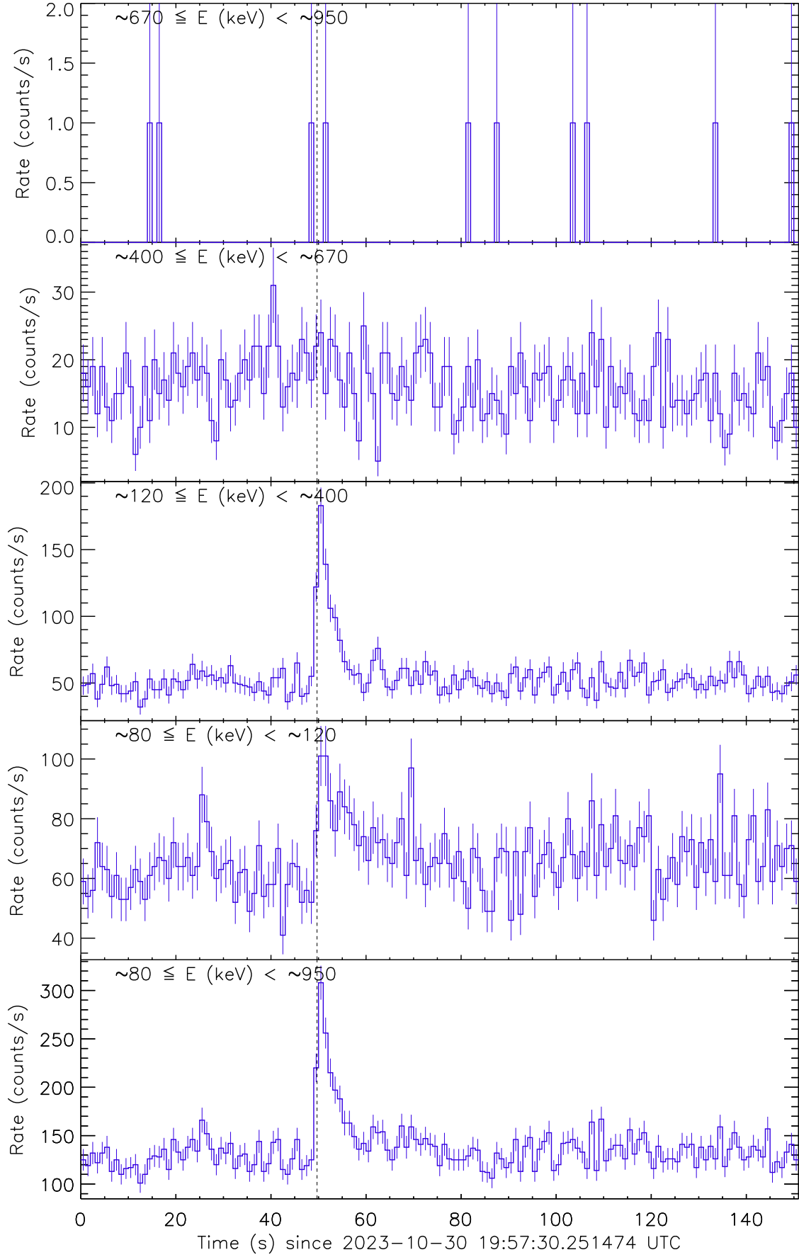
Figure 1: Raw count rate curve of GRB 231030B. The vertical dashed line marks the trigger time by Fermi/GBM.
