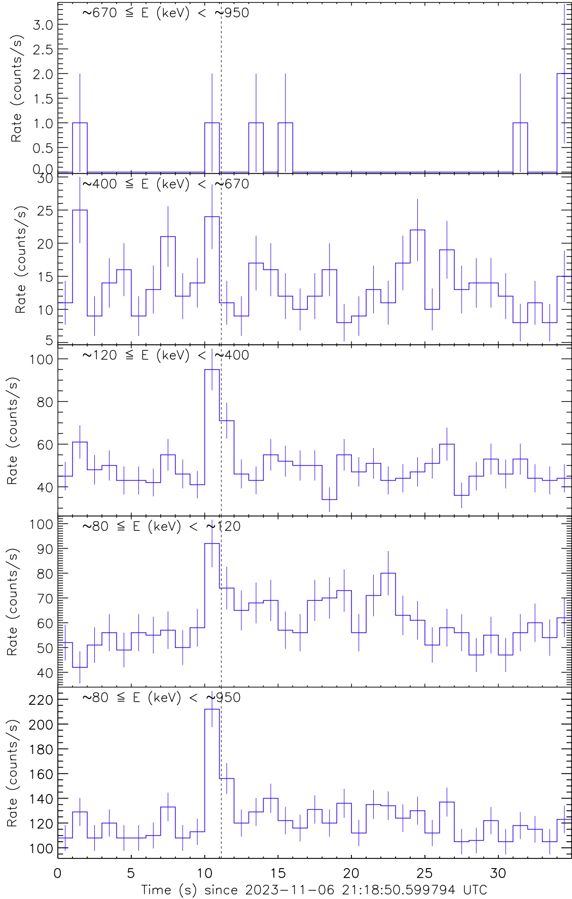
Figure 1: Raw count rate curve of GRB 231106B. The vertical dashed line marks the trigger time by Konus/Wind.
