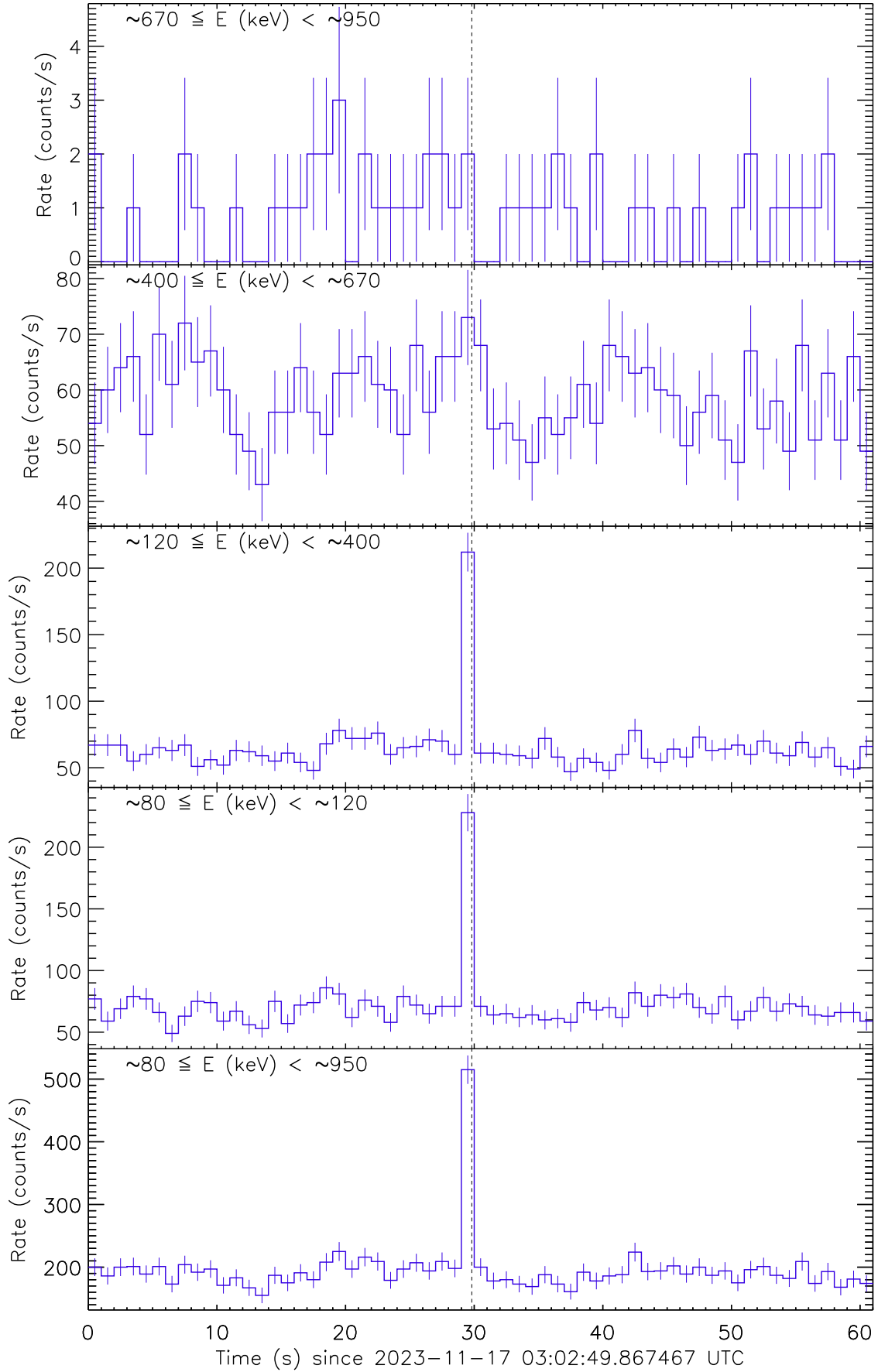
Figure 1: Raw count rate curve of GRB 231117A. The vertical dashed line marks the trigger time by AstroSat.
