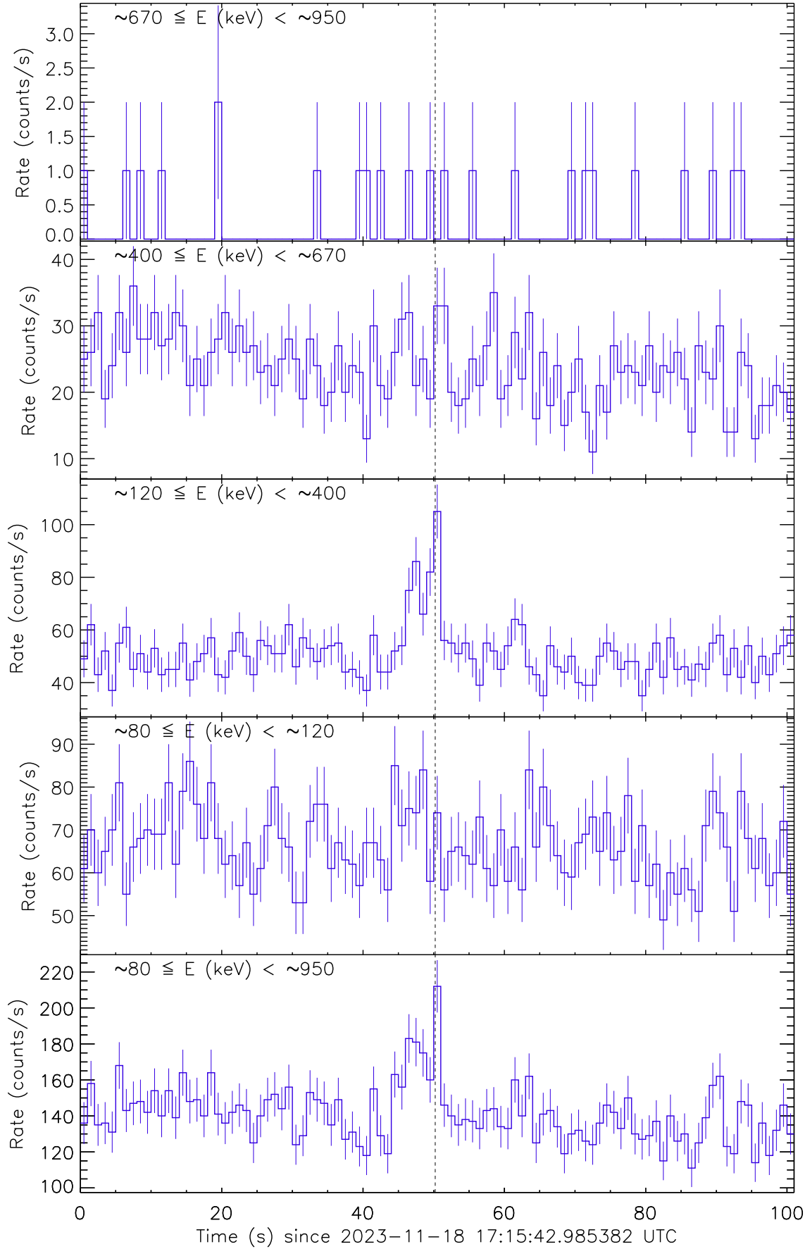
Figure 1: Raw count rate curve of GRB 231118A. The vertical dashed line marks the trigger time by Swift/BAT.
