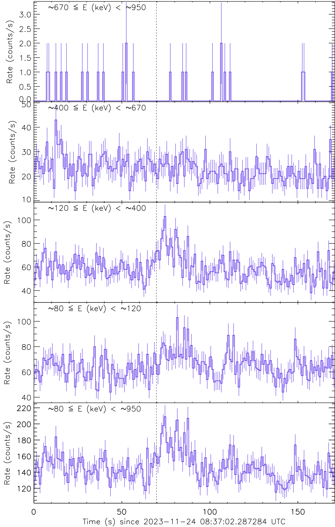
Figure 1: Raw count rate curve of GRB 231124A. The vertical dashed line marks the trigger time by Fermi/GBM.
