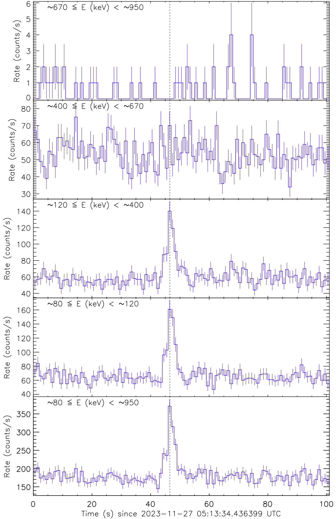
Figure 1: Raw count rate curve of GRB 231127A. The vertical dashed line marks the trigger time by AstroSat.
