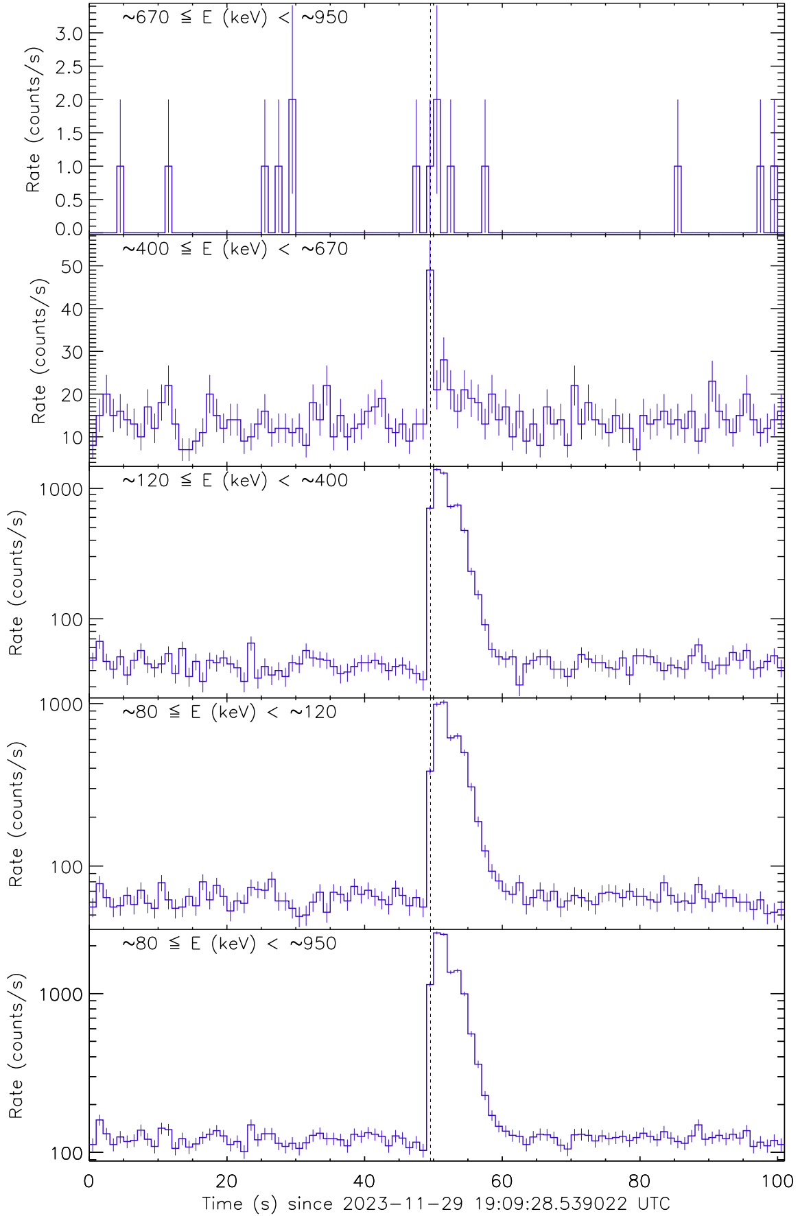
Figure 1: Raw count rate curve of GRB 231129C. The vertical dashed line marks the trigger time by Fermi/GBM.
