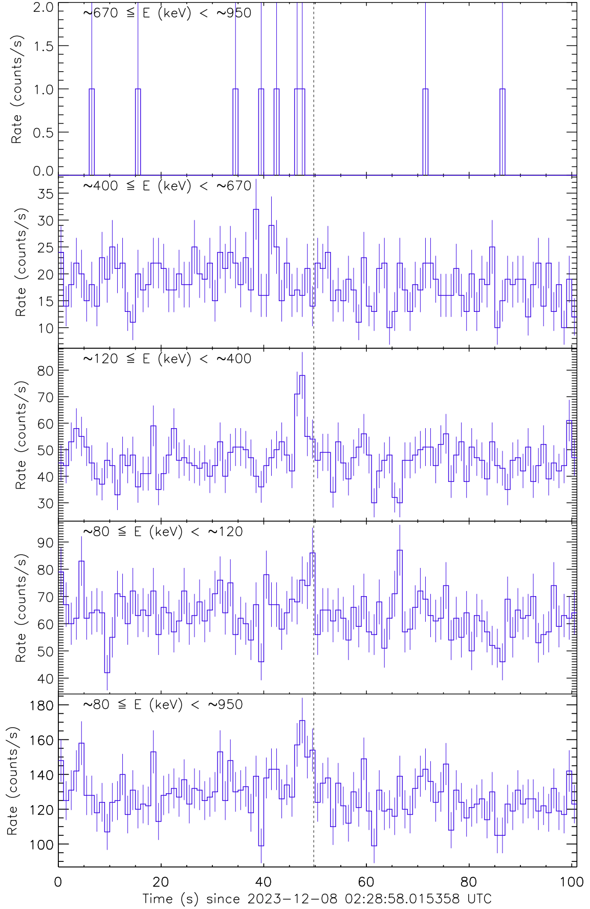
Figure 1: Raw count rate curve of GRB 231208A. The vertical dashed line marks the trigger time by AstroSat.
