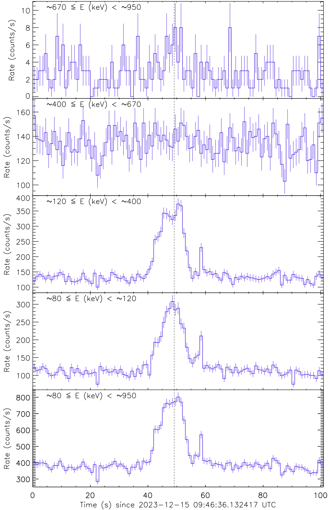
Figure 1: Raw count rate curve of GRB 231215A. The vertical dashed line marks the trigger time by Swift/BAT.
