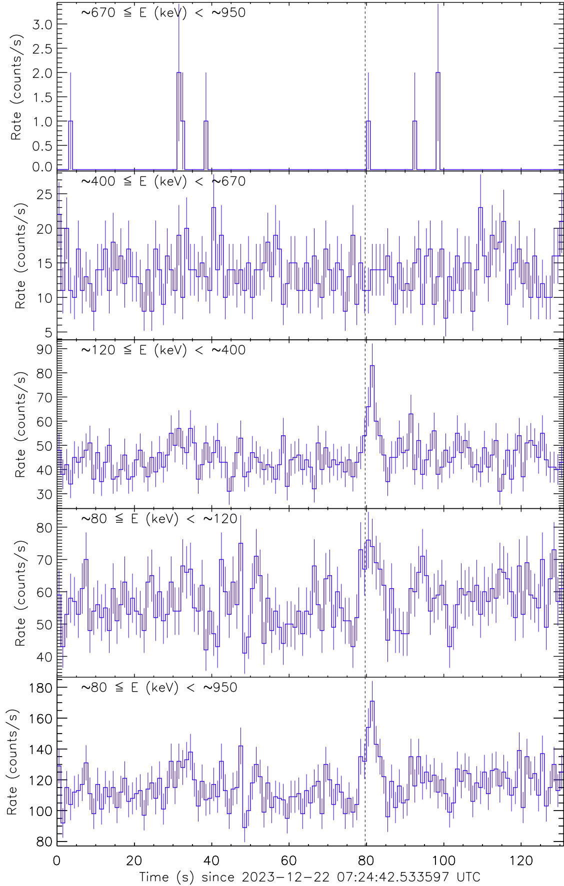
Figure 1: Raw count rate curve of GRB 231222B. The vertical dashed line marks the trigger time by Fermi/GBM.
