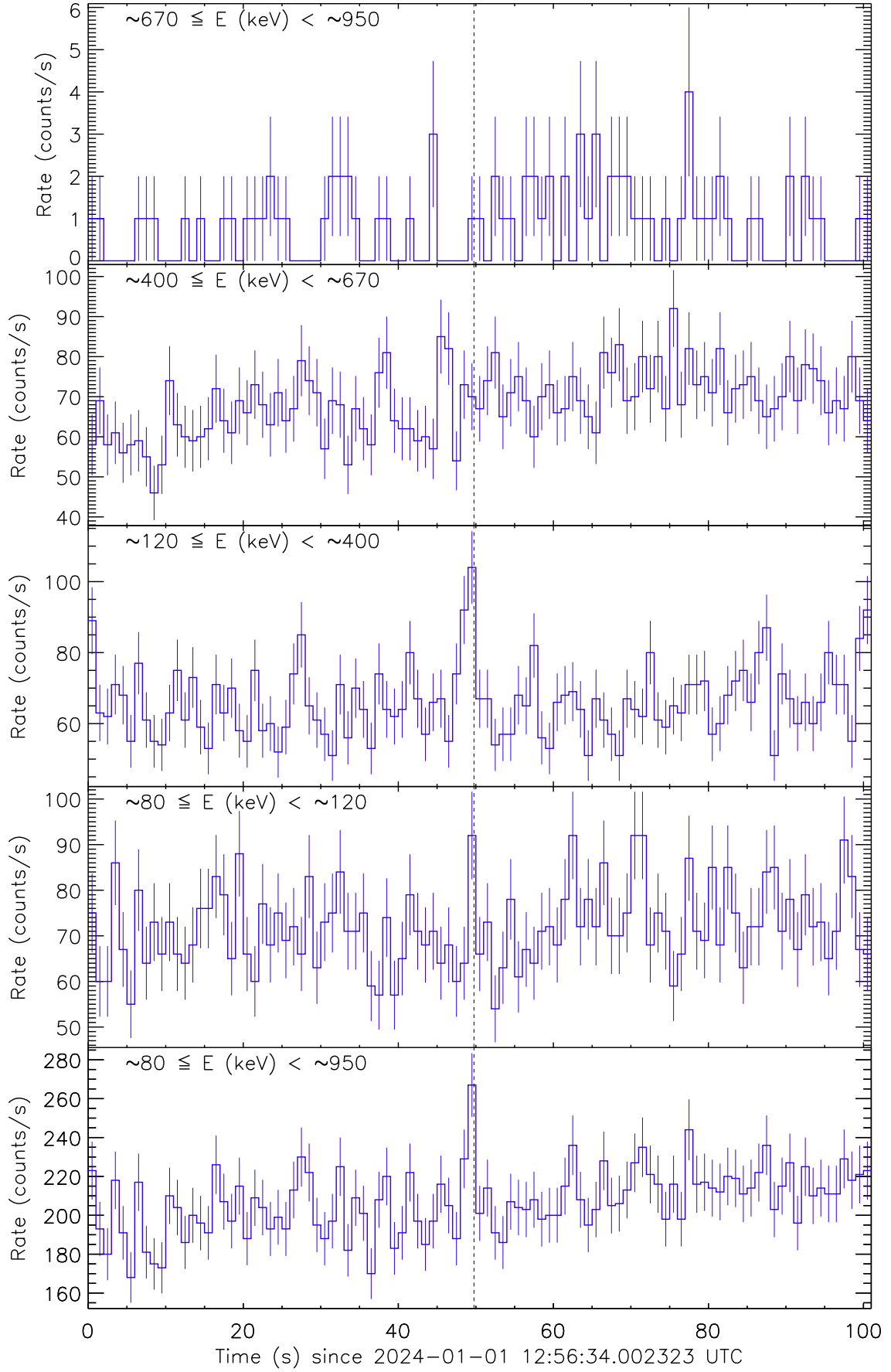
Figure 1: Raw count rate curve of GRB 240101C. The vertical dashed line marks the trigger time by Fermi/GBM.
